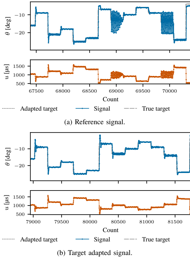
Fig. 12: Qualitative comparison of 1min of the signal response for the slow-aggressive PID controller.
