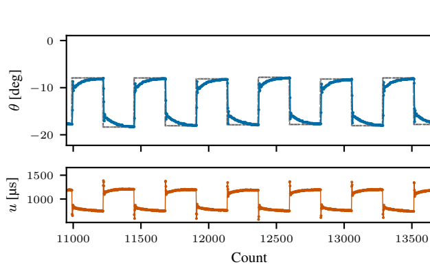
(a) Reference signal.
