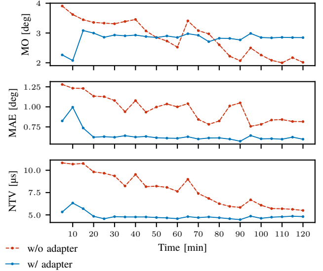
Fig. 16: Metrics evolution over the 2h duration of the experiment for an aggressive but under-responsive PID controller. Each point represents the calculated value of the metric on identical 5min sequences of targets. Plots for all metrics and numerical values can be found in Figure C.1 and Table C.I, respectively.
