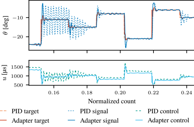
Fig. 15: Qualitative comparison between the behavior of the baseline controller and target adapted controller for the slow-aggressive PID controller.
