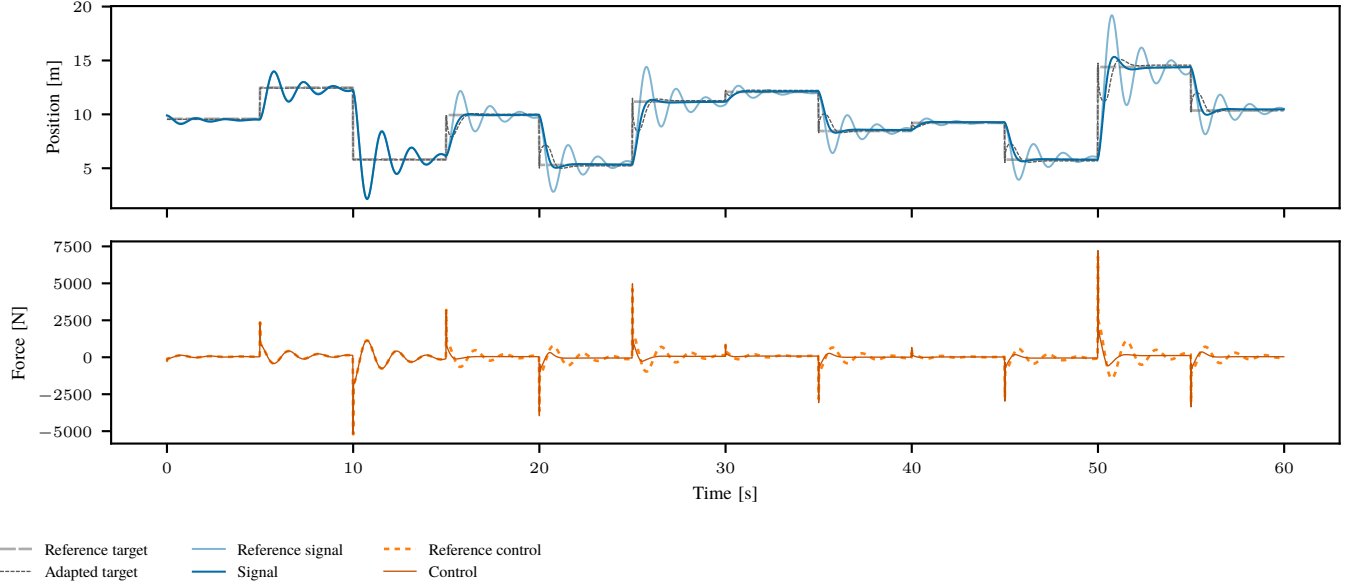
Fig. 4: The full minute simulation of the toy problem. Top: The system response x and target x_d + \Delta of the adapted controller, alongside the response and target of the unadapted reference controller ( \Delta = 0 ). Bottom: The resulting adapted control inputs from the controller receiving x_d + \Delta alongside the unaltered reference control inputs. During the first 15 seconds (3 targets) the adapter has not received updates yet, and the signal is thus identical to the reference signal.
