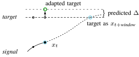
Fig. 2: Target adaptation during deployment: By supplying the model with the controller’s target as x_{t+window} it yields a \Delta that can be added to the current target, which will supposedly result in the controller reaching the target within the specified window.
