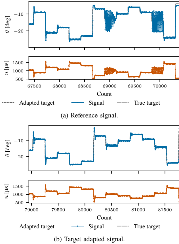
Fig. 12: Qualitative comparison of 1min of the response signal for the slow-aggressive PID controller.
