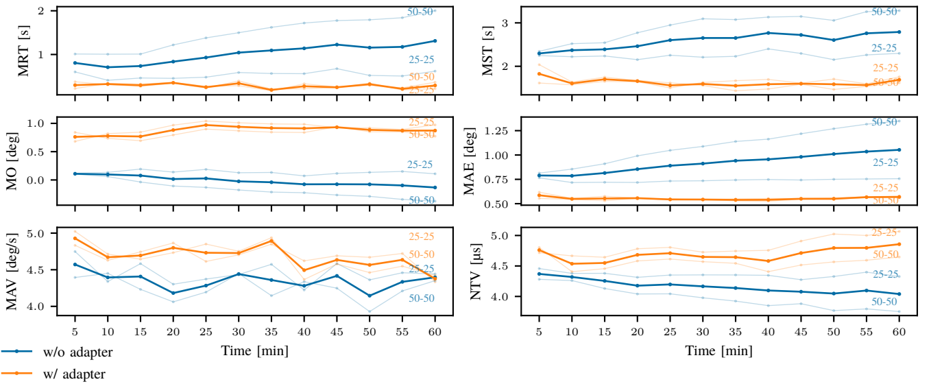
Fig. 16: Metrics evolution over the 1h duration of the experiment for KOSs in a lower state of degradation (0.25–0.25mm and 0.5–0.5mm perforations, see annotations), with their average overlaid. Each point represents the calculated value of the metric on identical 5min sequences of targets. Numerical values can be found in Appendix C.
