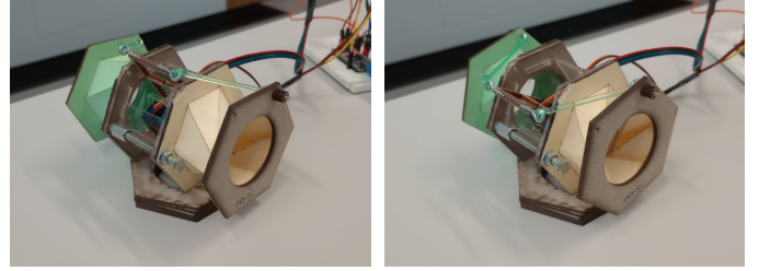
Fig. 12: Top : The “feet” of the robot grip when dragged backwards, but slide when pushed forward, allowing the robot to move forward, also known as two-anchor crawling (Calisti et al., 2017). Left : The robot at its fully extended state, corresponding to the “home” position of the servo and actuation arm. Right : The fully contracted robot, corresponding to the maximum (capped) servo output, near the mechanical limit of the actuation arm.
