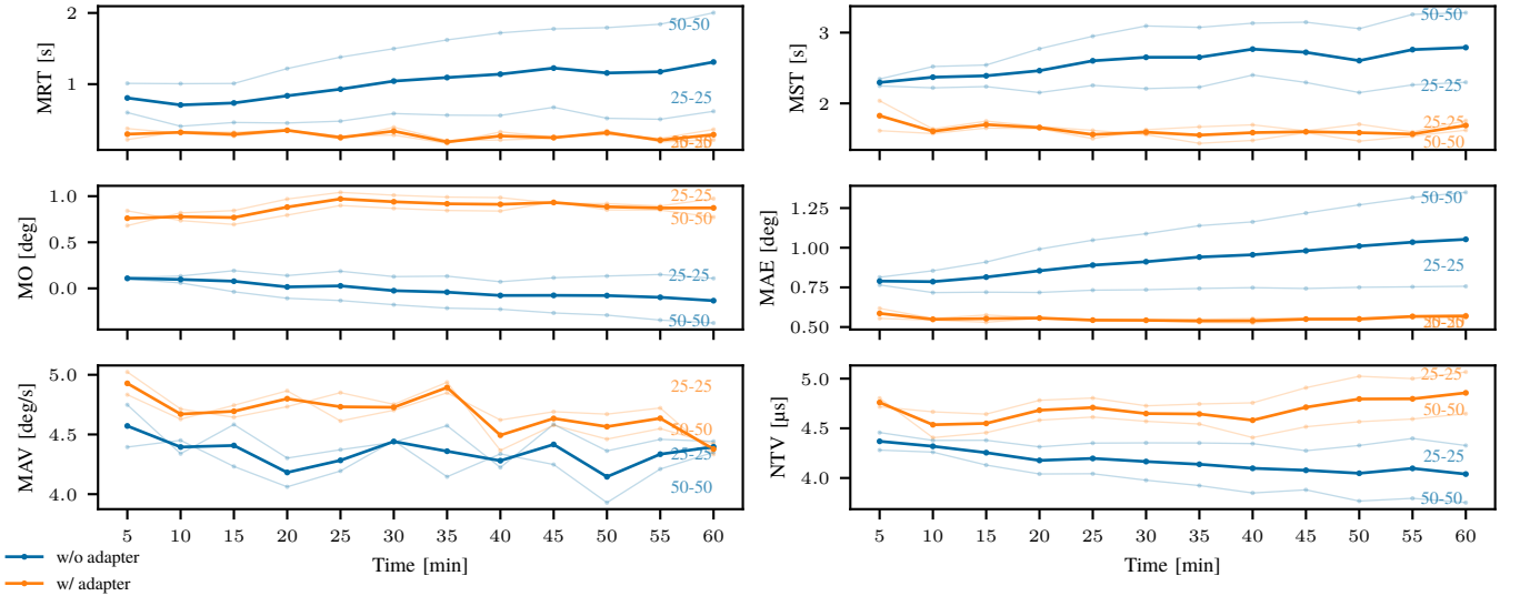
Fig. 16: Metrics evolution over the 1h duration of the experiment for KOSs in a lower state of degradation (0.25–0.25mm and 0.5–0.5mm perforations, see annotations), with their average overlayed. Each point represents the calculated value of the metric on identical 5min sequences of targets. Numerical values can be found in Appendix C.
