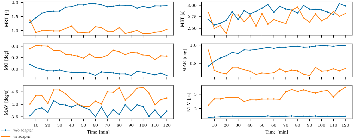
Fig. 15: Metrics evolution over the duration of the experiment for an under-tuned PID controller. Each point represents the calculated value of the metric on identical 5min sequences of targets. Numerical values can be found in Appendix C.
