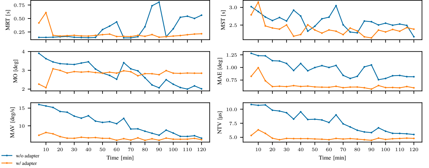
Fig. 13: Metrics evolution over the 2h duration of the experiment for an aggressive but under-responsive PID controller. Each point represents the calculated value of the metric on identical 5min sequences of targets. Numerical values can be found in Appendix C.
