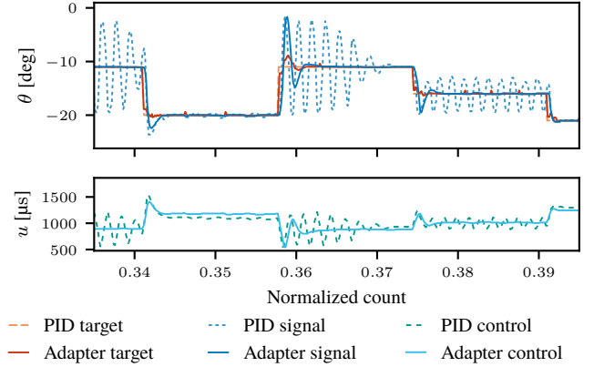
Fig. 15: Qualitative comparison between the behavior of the baseline controller and target adapted controller for the slow-aggressive PID controller.
