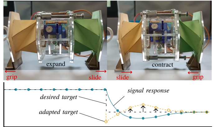
Fig. 1: The Kresling origami robot with target adaptation. Top: The “feet” of the robot grip when dragged backward, but slide when pushed forward, allowing the robot to move forward, also known as two-anchor crawling (Calisti et al., 2017). Bottom: The contraction target is adapted to reduce overshoot and unstable oscillations.
