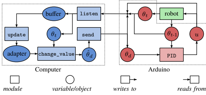
Fig. B.1: The interaction between the modules (rectangles) and shared variables (ovals) of the computer (blue) and Arduino (red).
