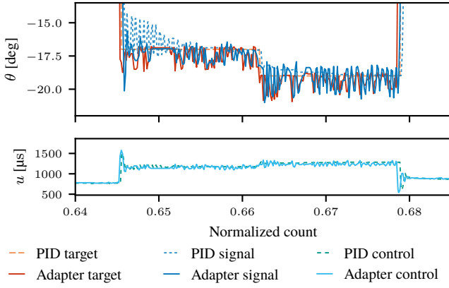
Fig. 27: A close-up of the 2–0.5mm experiment. The oscillations in the signal response are recorded at an insufficient frequency to contain any meaningful relationship between spaced-out state pairs and the target. As a result, the adapter’s output becomes more chaotic as well, further polluting the training data.
