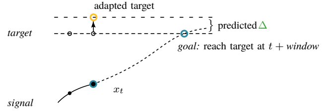
(a) By supplying the model with the controller’s target position and current state x_t , it yields a \Delta that can be added to the current target, which will supposedly result in the controller reaching the target within the specified window.
