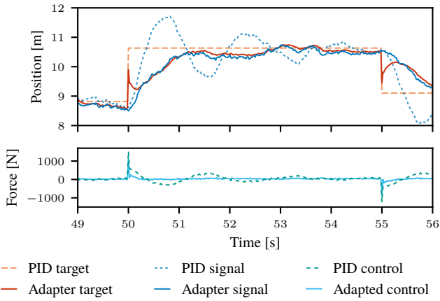
Fig. 8: A close-up of the second to last target in the one-minute simulation. The effects of the adapter can be more clearly observed: The overshoot (seen in the baseline PID signal) is countered by bringing the target closer to the current state.
