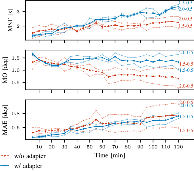
Fig. 21: Metrics evolution over the 2h duration of the experiment for KOSs in a higher state of degradation (1.5–0.5mm and 2–0.5mm perforations, see annotations), with their average overlayed. Each point represents the calculated value of the metric on identical 5min sequences of targets. Plots for all metrics and numerical values can be found in Figure C.4 and Table C.IV, respectively.
