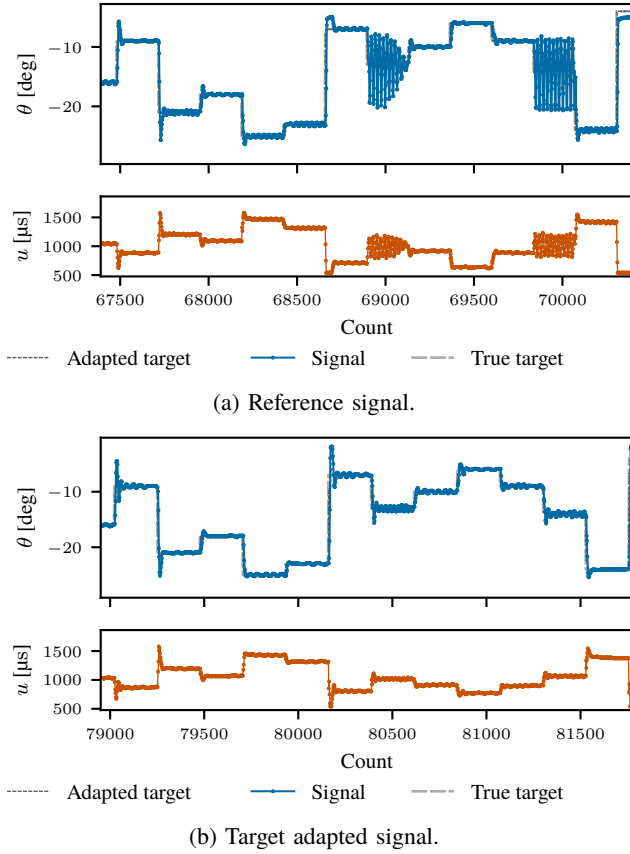
Fig. 13: Qualitative comparison of 1min of the signal response for the slow-aggressive PID controller.
