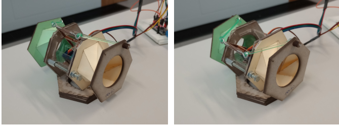
Fig. 10: Left : The robot at its fully extended state, corresponding to the “home” position of the servo and actuation arm. Right : The fully contracted robot, corresponding to the maximum (capped) servo output, near the mechanical limit of the actuation arm.
