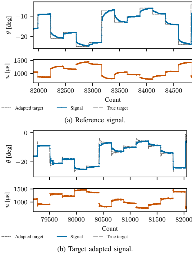
Fig. 15: Qualitative comparison of 1min of the signal response for the under-tuned PID controller.
