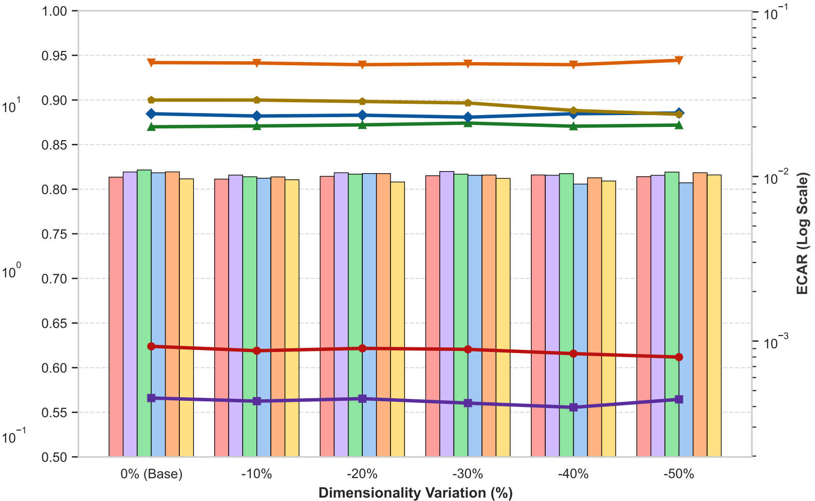
Dataset: German
