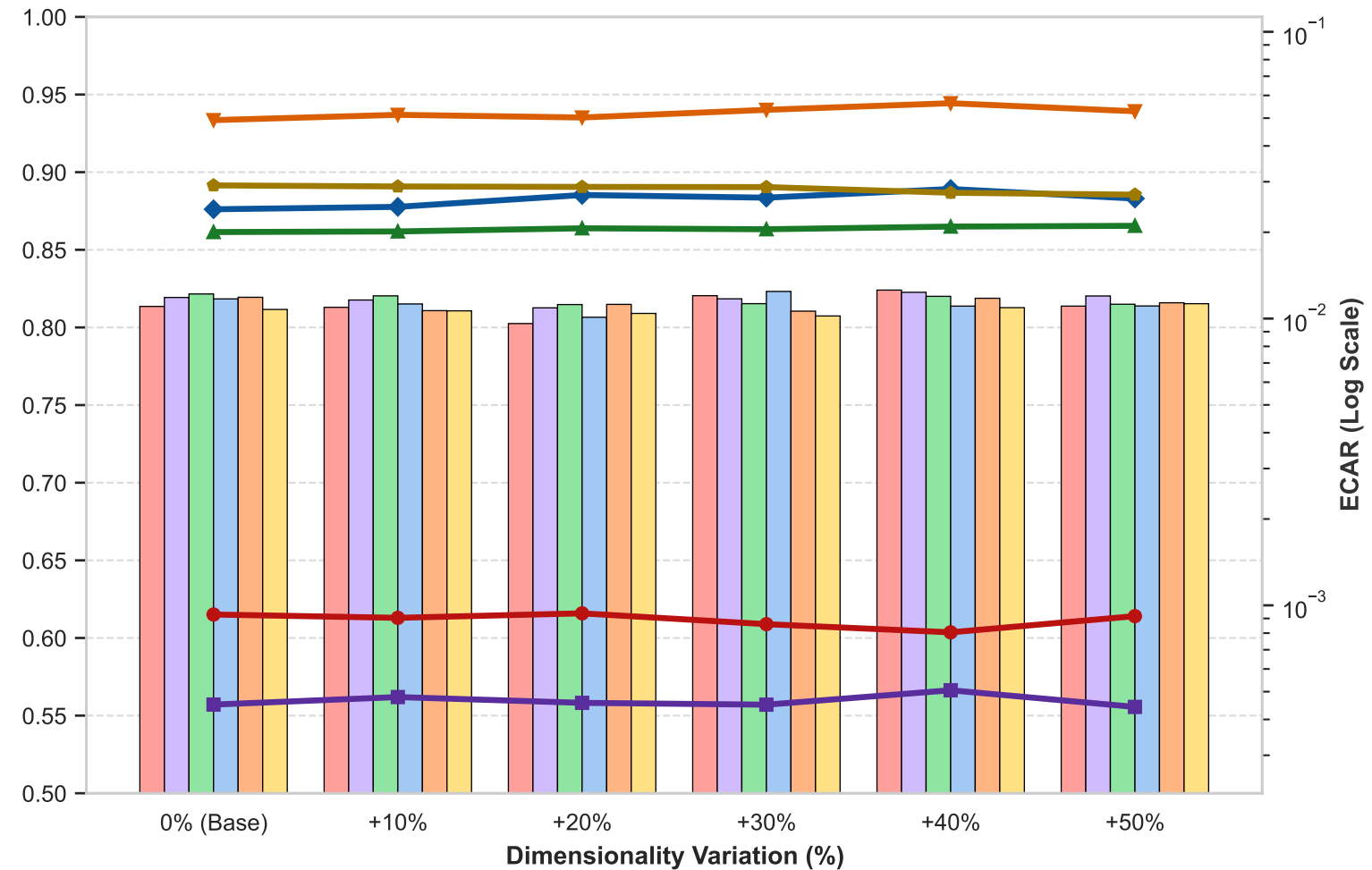
Dataset: German
