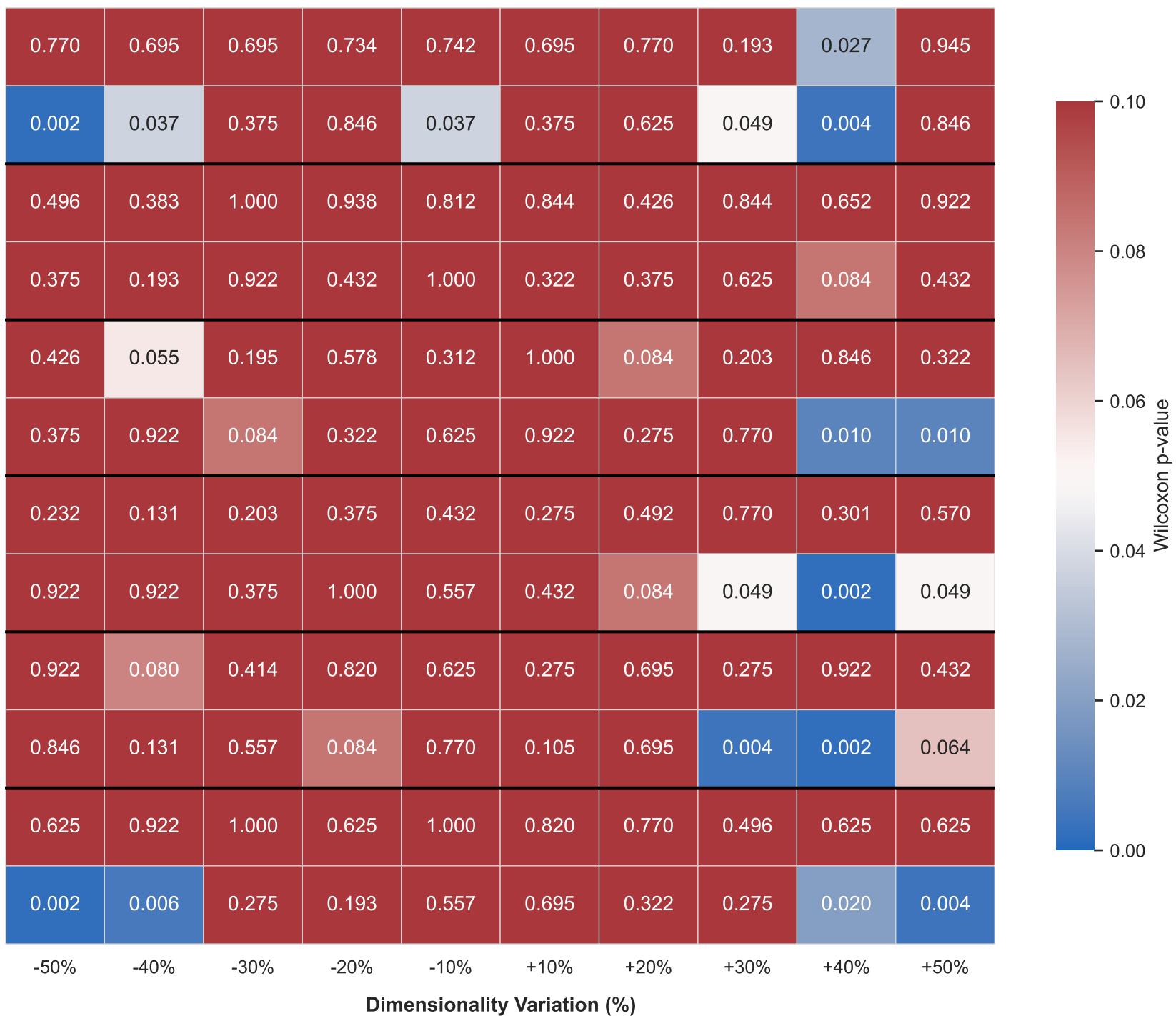
Dataset: German
