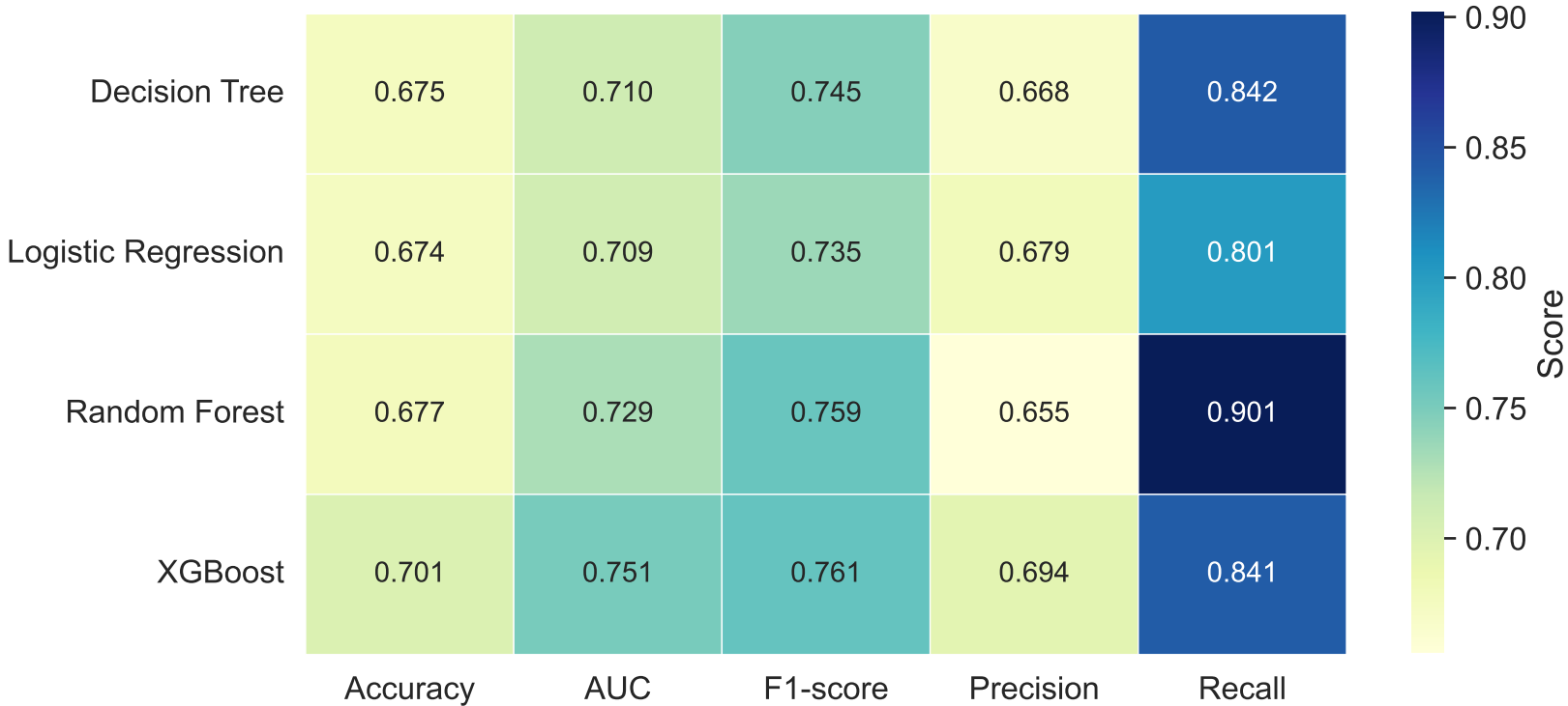
Predictive Performance (All 4 Features Removed)
