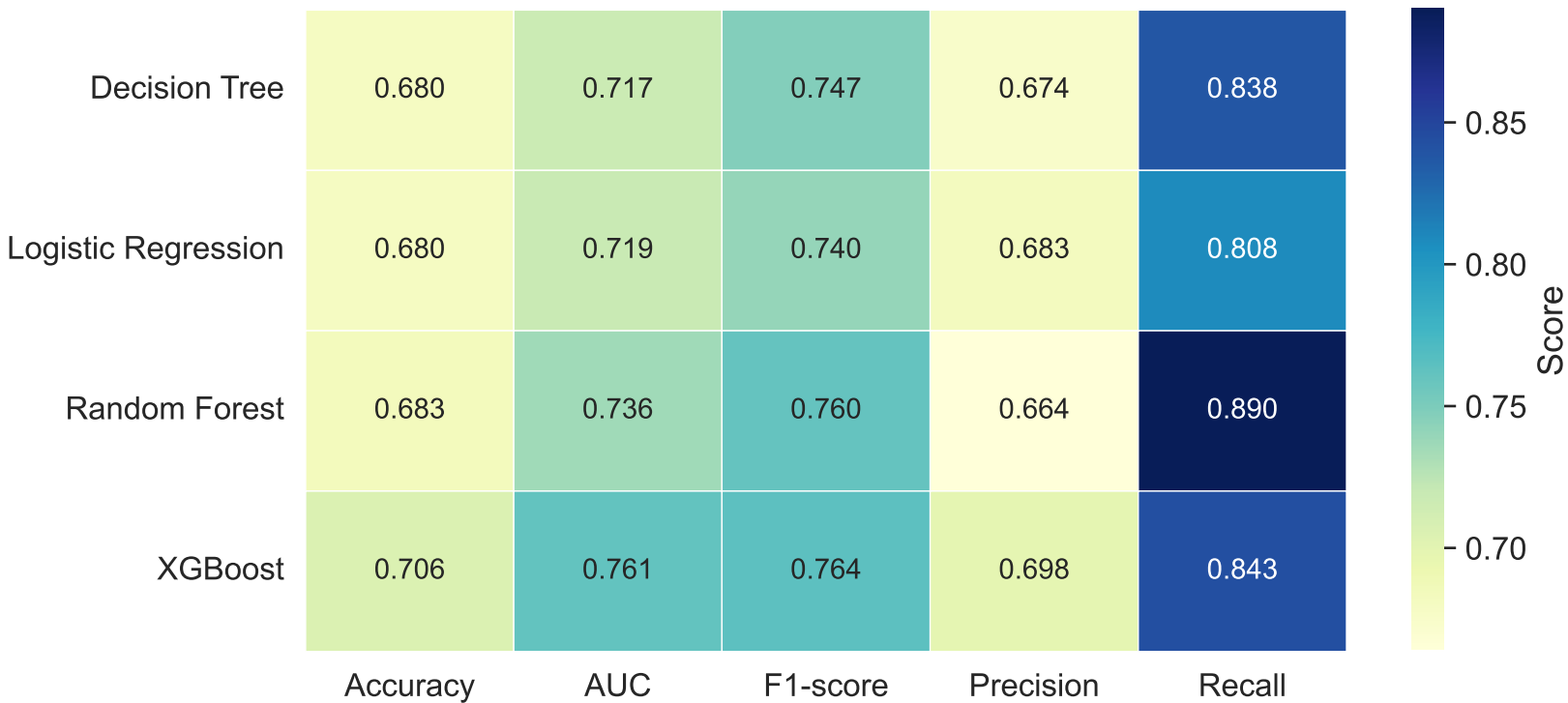
Predictive Performance (Removed Feature: MaritalStatus)
