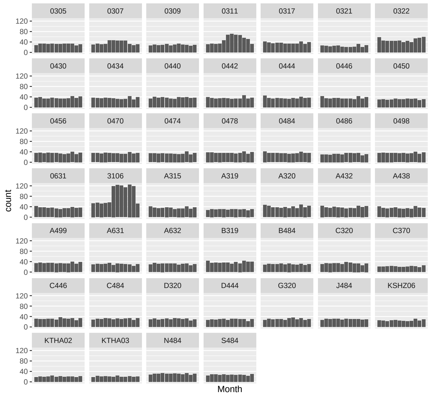
NO2-3, Monthly Readings by Locator, 1979-2008
