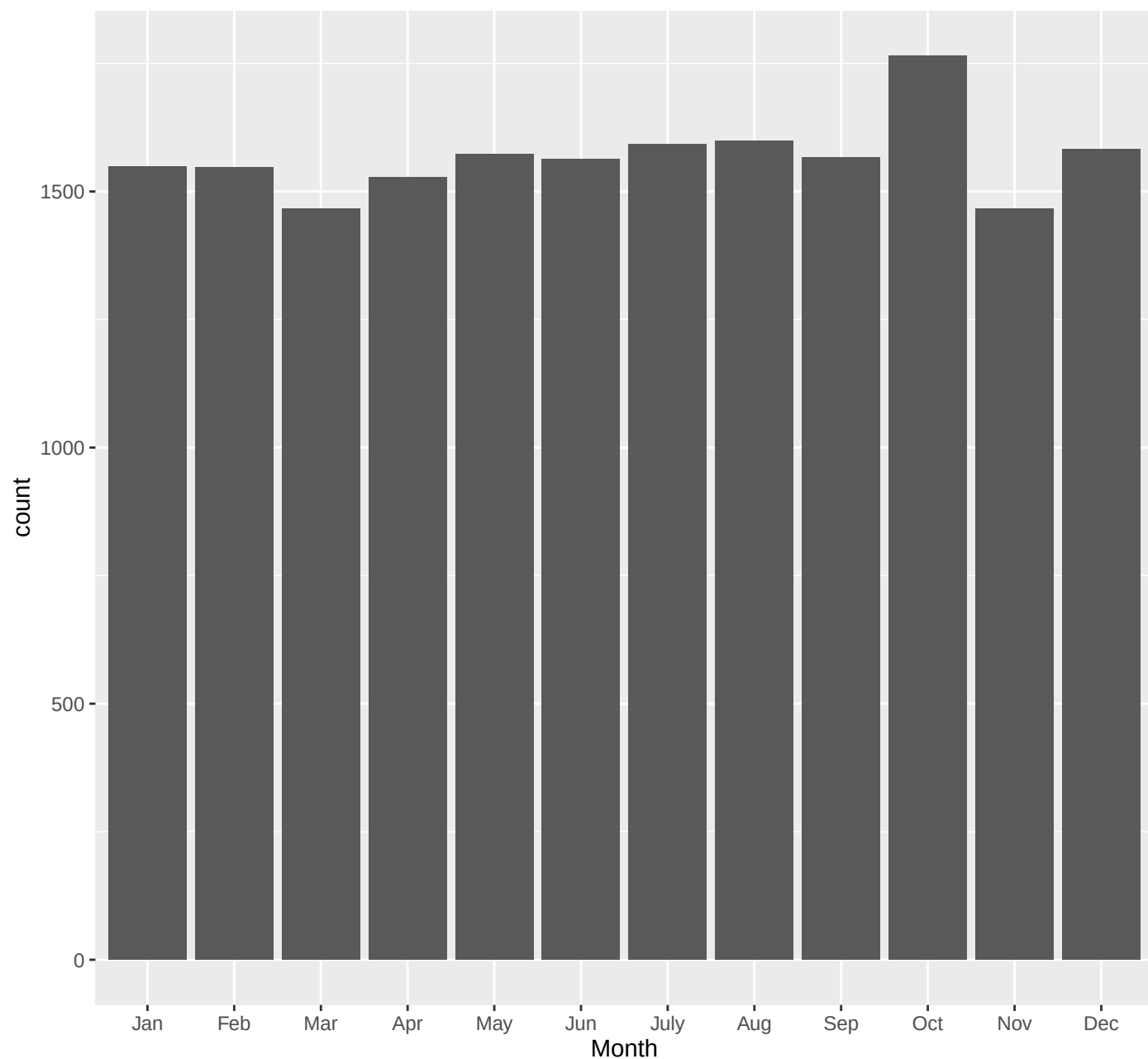
NO 2 -3, Monthly Readings, 1979–2008
