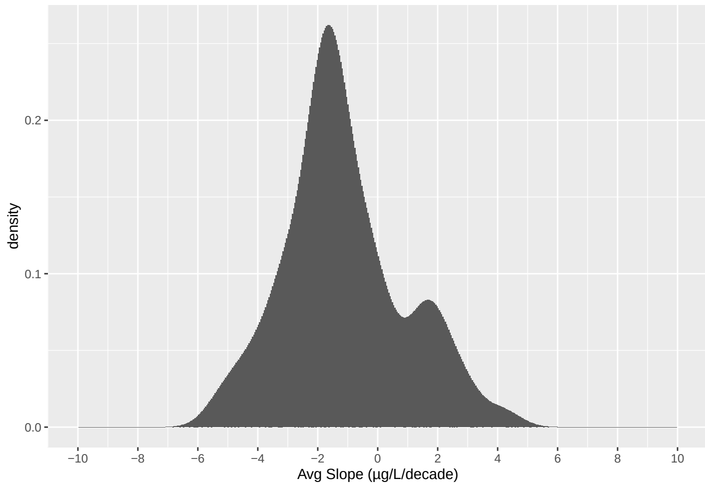
PO4 Slope Distribution Curve, Zoomed-in
