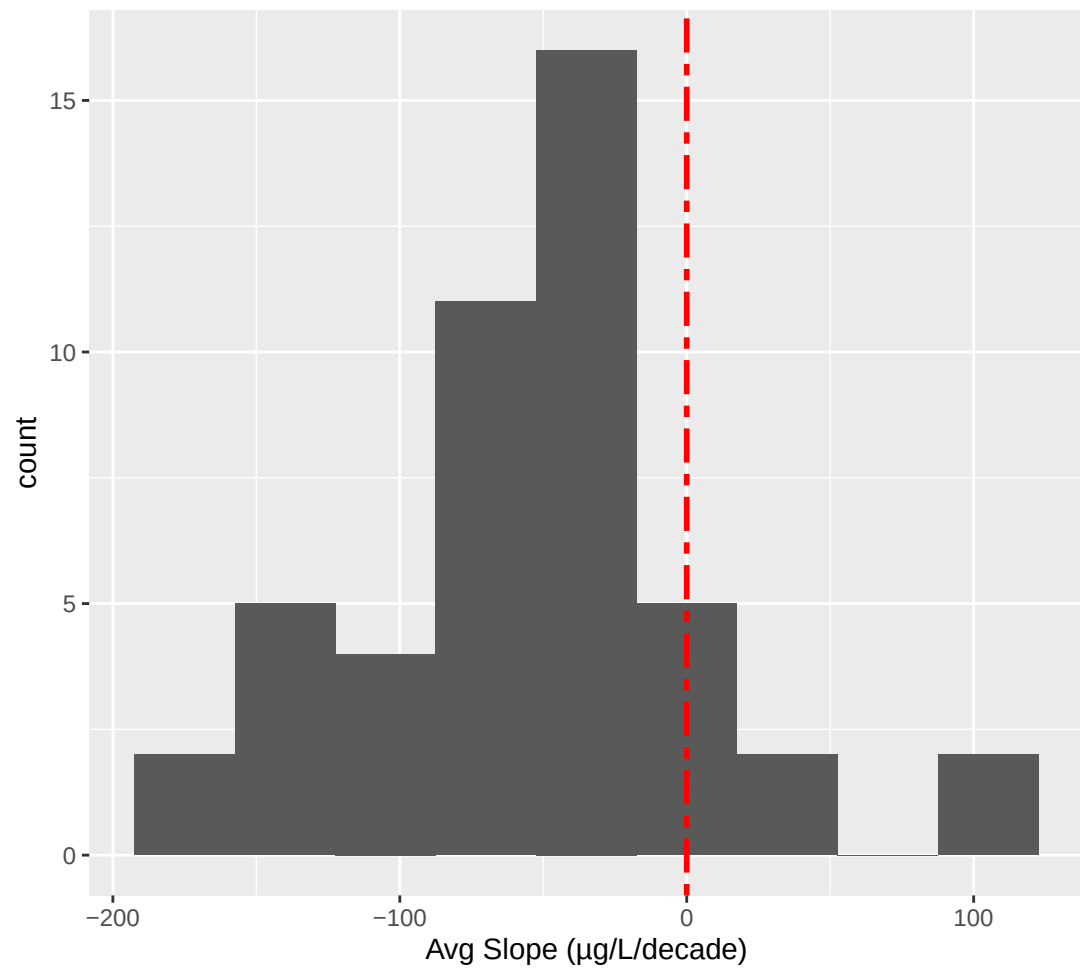
NO2/3 Slope Distribution Histogram Option 3, bin-width = 35
