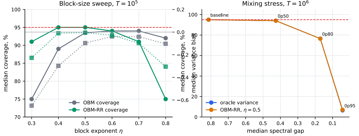
Figure 2: Left: block-size sensitivity of OBM and OBM-RR at T = 10^5 . Right: slow-mixing stress test at T = 10^6 , comparing oracle variance intervals with OBM-RR intervals at \eta = 0.5 .
