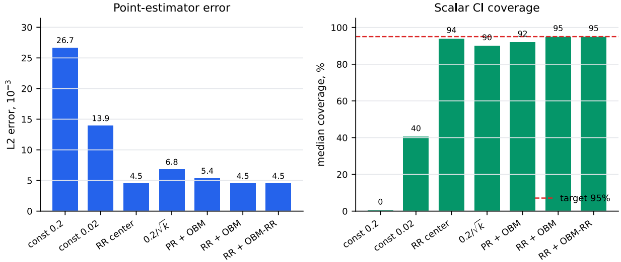
Figure 1: Main comparison at T = 10^6 . The left panel shows median Euclidean error and the right panel shows median scalar coverage across the same 100 generated problems.
