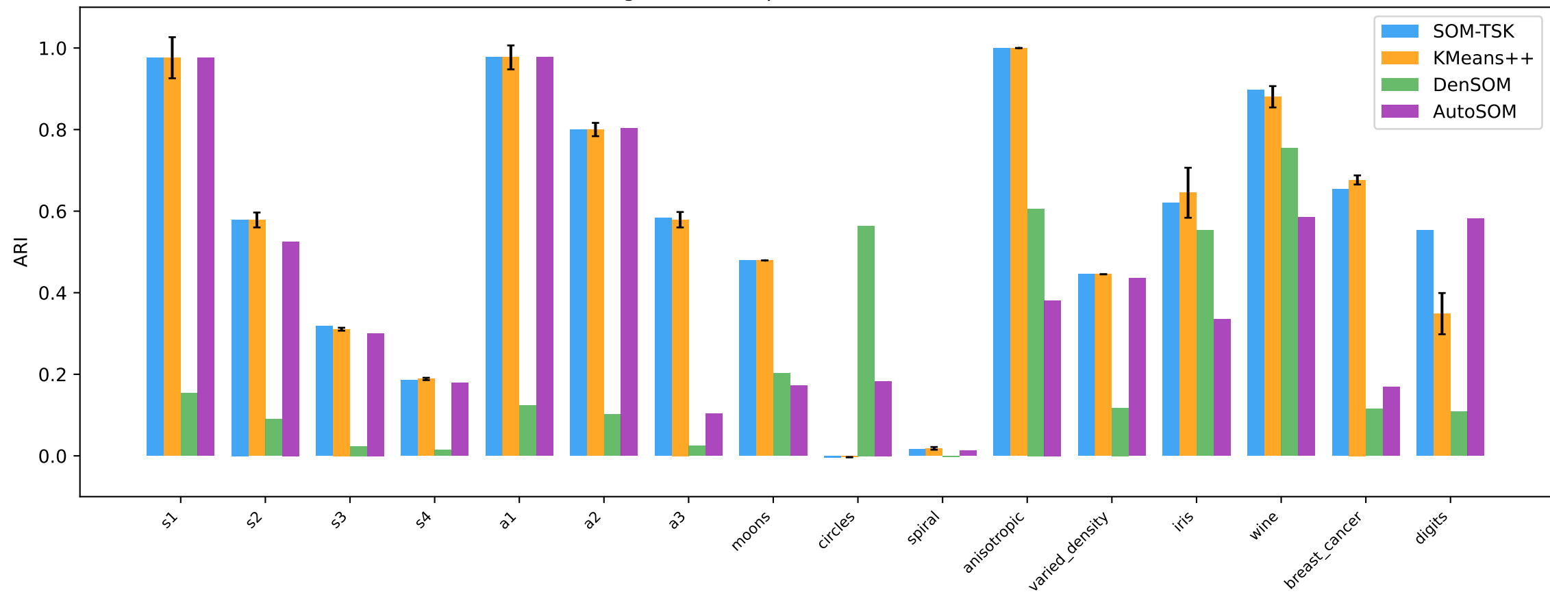
Algorithm Comparison Across Datasets
