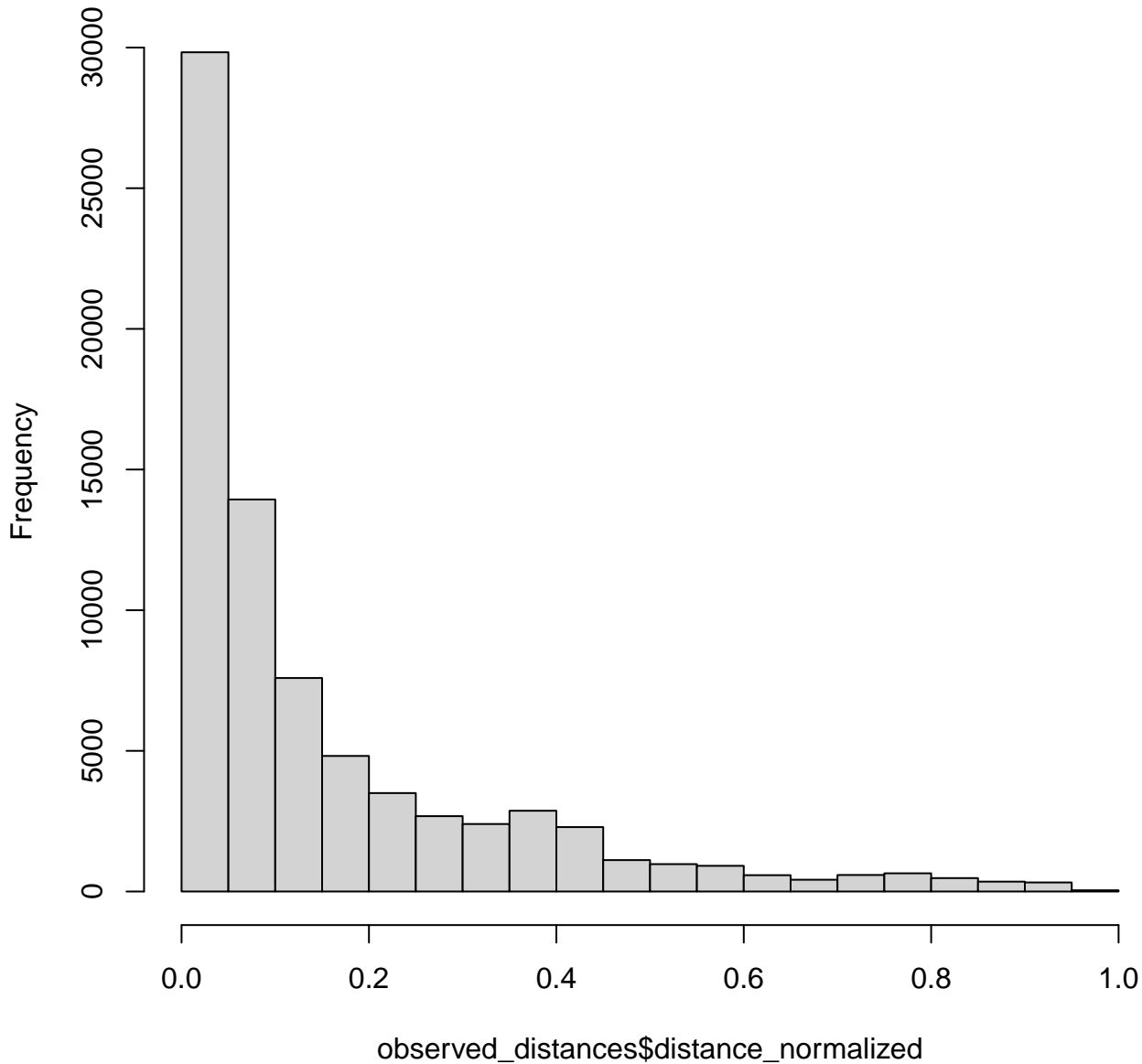
Histogram of observed_distances$distance_normalized
