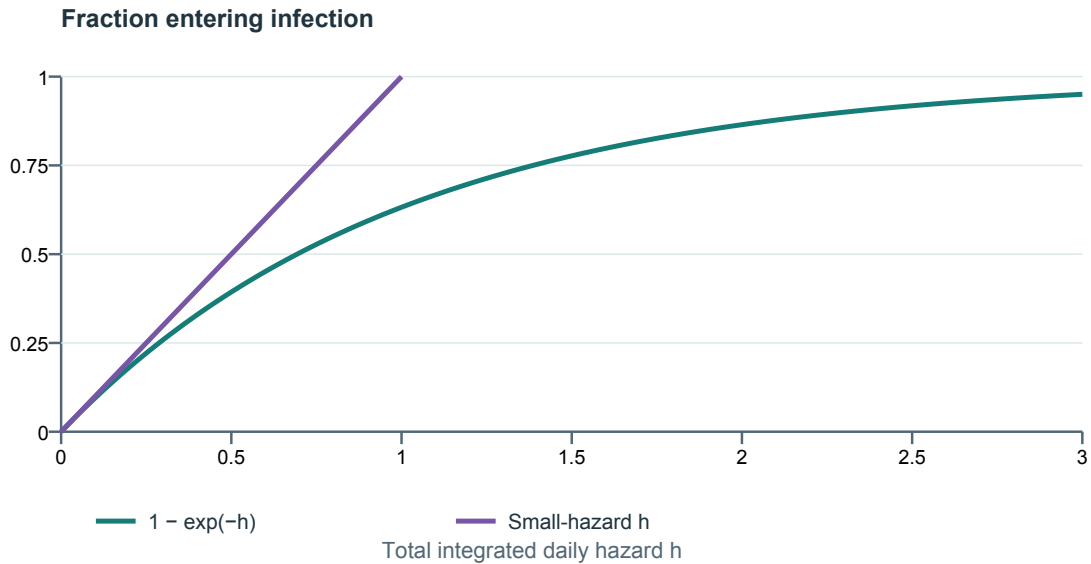
Figure 2: The infection entry fraction and its linear approximation at small hazard.
