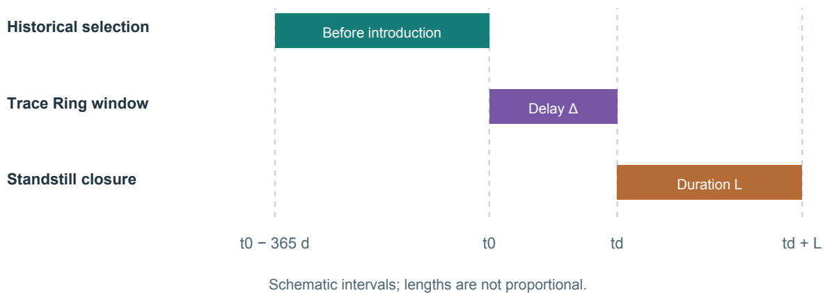
Figure 4: Historical selection, tracing, response and reopening use distinct calendar intervals.
