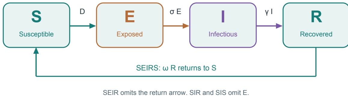
Figure 1: Compartment transitions. Every arrow uses the state at the start of the same day.
