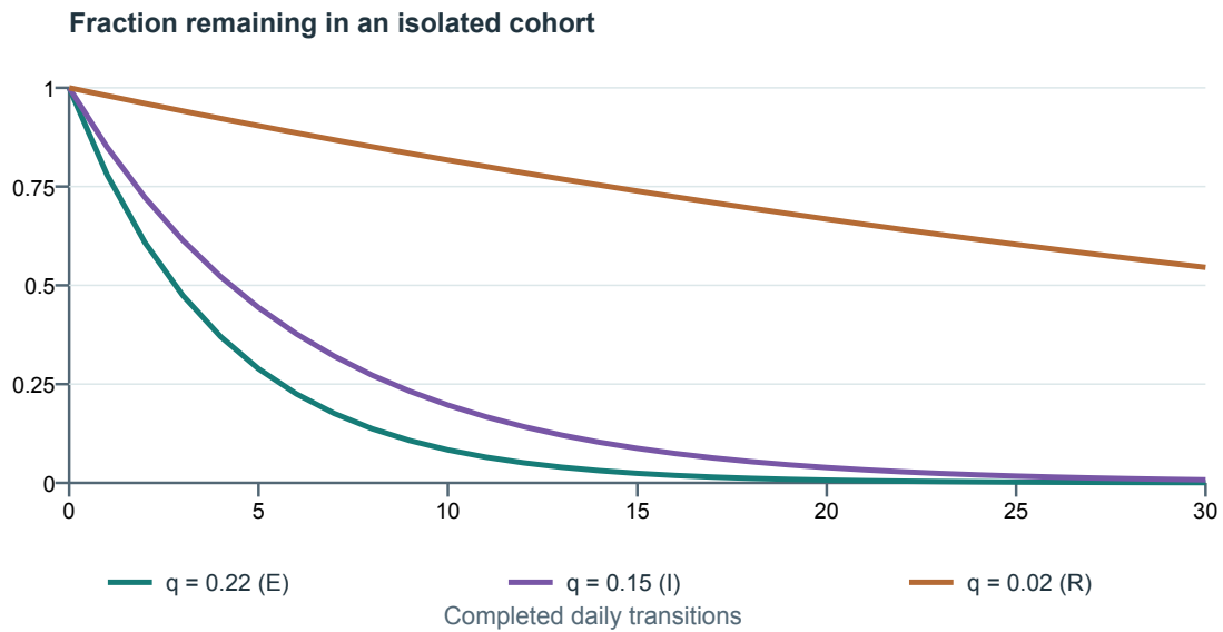
Figure 3: Surviving fractions under three daily exit fractions. A long tail is part of the compartment assumption.
