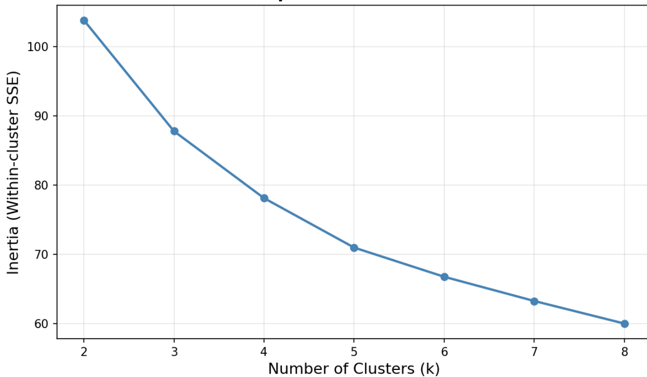
Figure: Elbow Method -- Optimal k Selection
