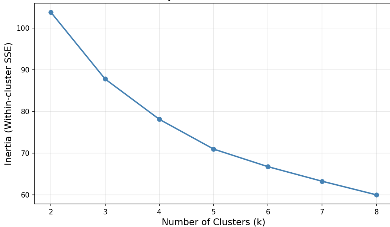
Figure: Elbow Method -- Optimal k Selection
