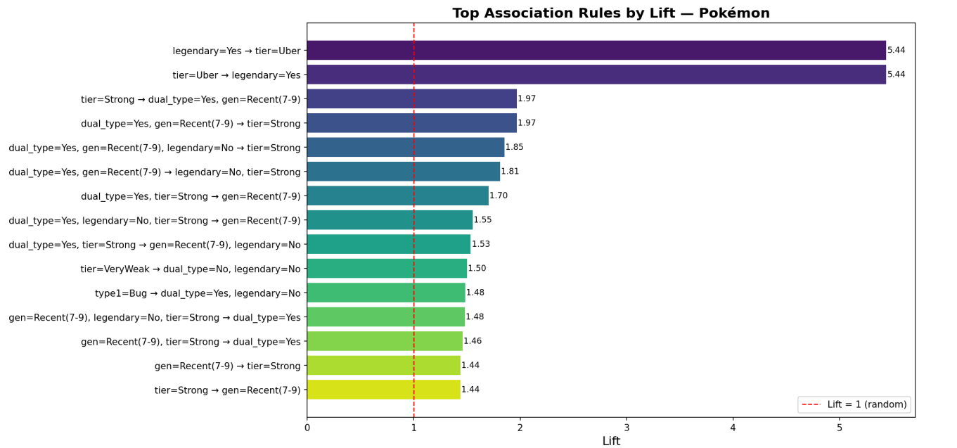
Figure: Top Association Rules by Lift
