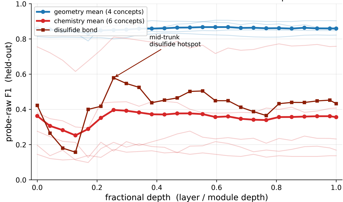
Pairformer trunk encodes both families of concept
