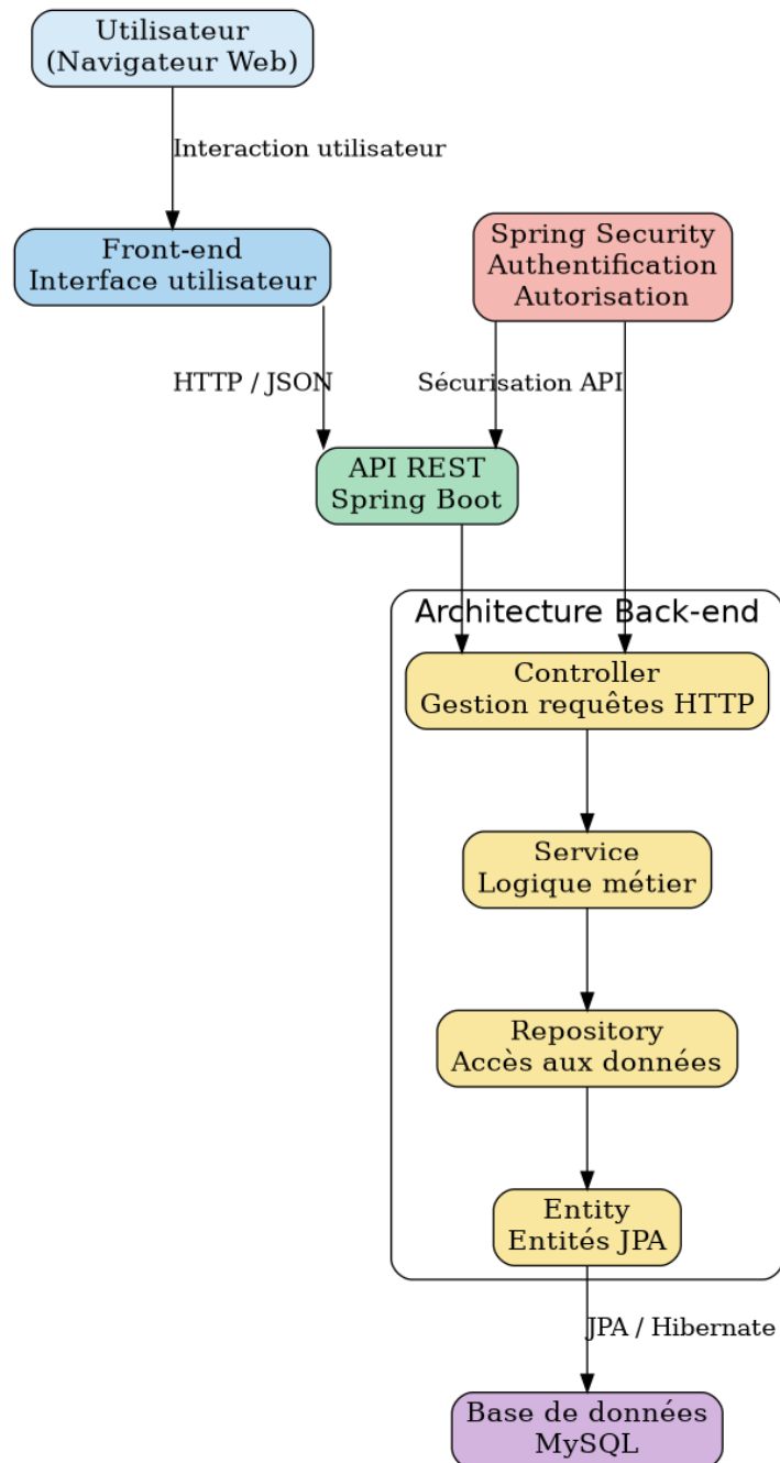
Figure 3 : Architecture technique de l'application One Piece RPG
