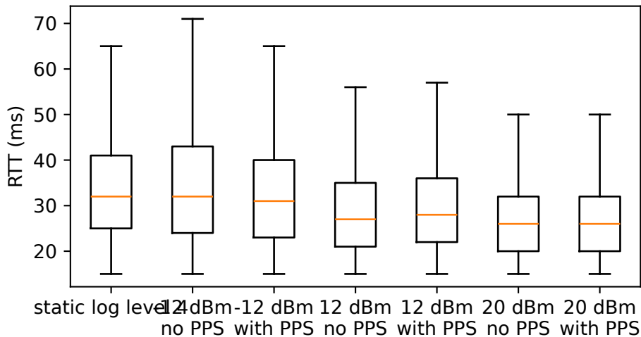
Ping to Parent Round-trip Time
