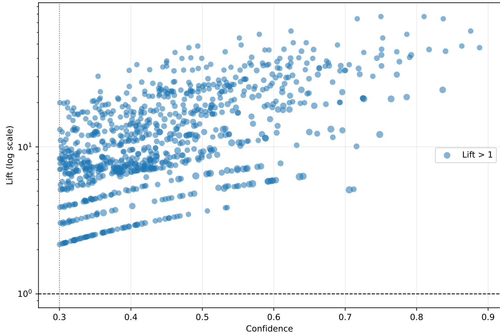
Confidence-lift relationship for interpretable rules
