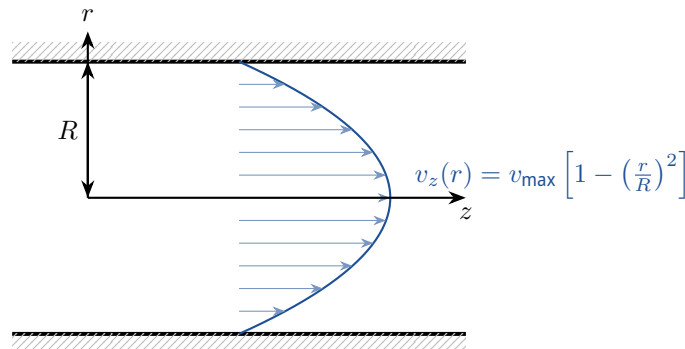
Figure 3: Parabolic velocity profile of Hagen-Poiseuille flow in a circular pipe.
