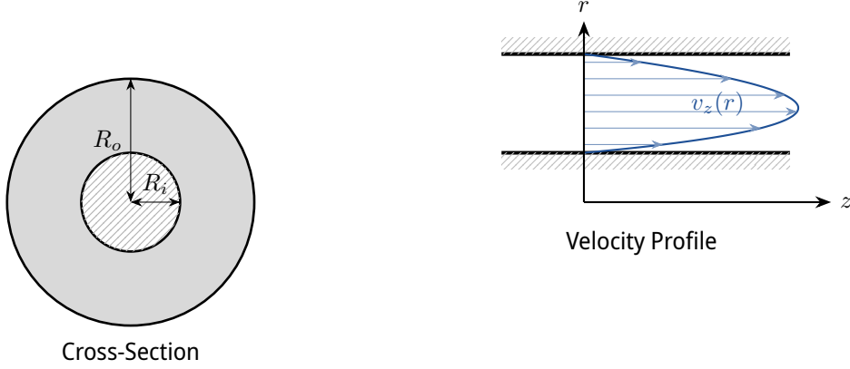
Figure 4: Geometry and velocity profile for laminar flow in a coaxial annulus.
