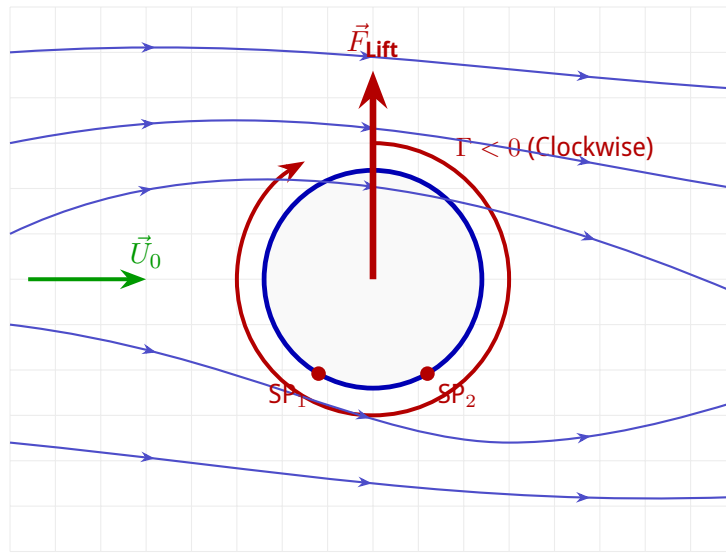
Figure 1: Streamlines and lift force for flow around a clockwise rotating cylinder (Magnus effect).
