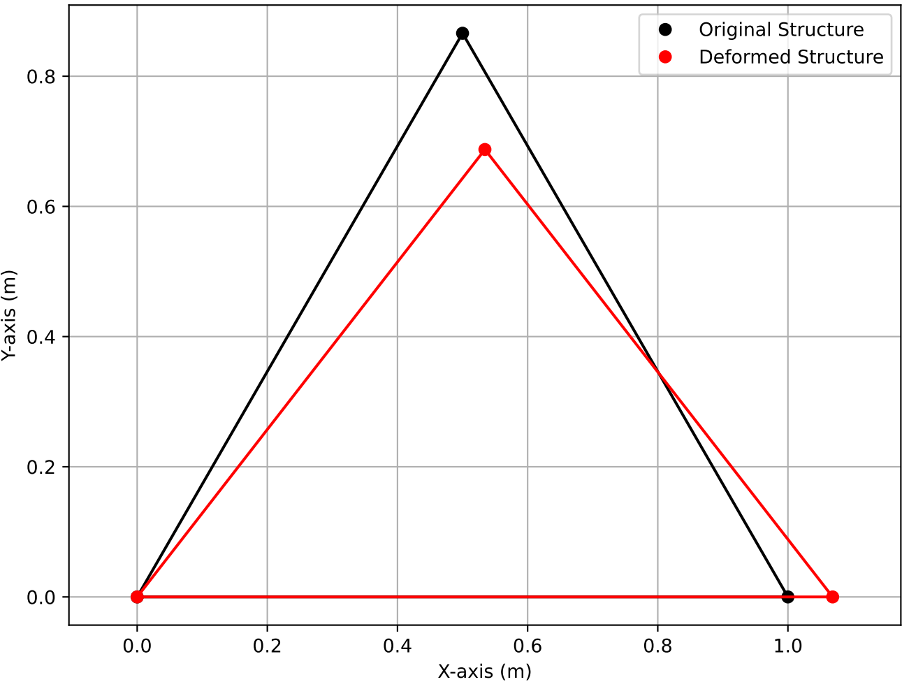
Three Bar Truss Deformation (Scale = 5.000000e+05)
