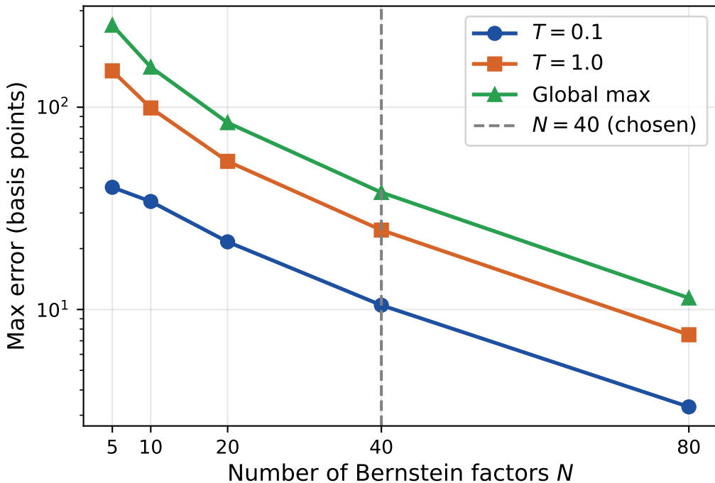
COS Pricer: Convergence in Bernstein Factors
