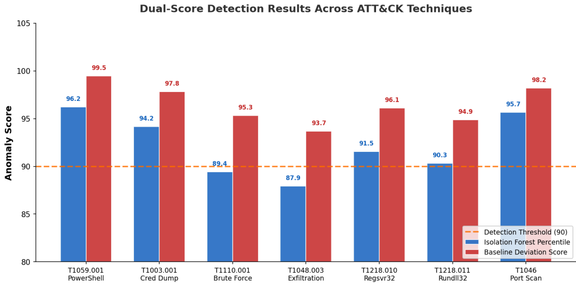
Figure 27: Comparative dual-score detection results across all tested ATT&CK techniques.
