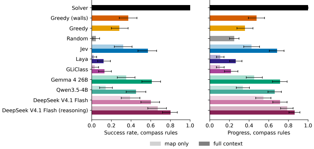
Figure 2: Success rate and progress under compass rules, with the map only (pale bars) and full context (dark bars). Lines show 95% intervals.
