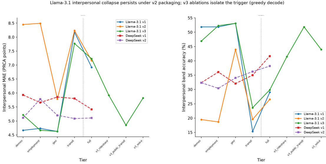
Figure 2. Llama-3.1 vs DeepSeek interpersonal MAE by tier across prompt-v1 (v1), v2, and v3 (greedy) exports
