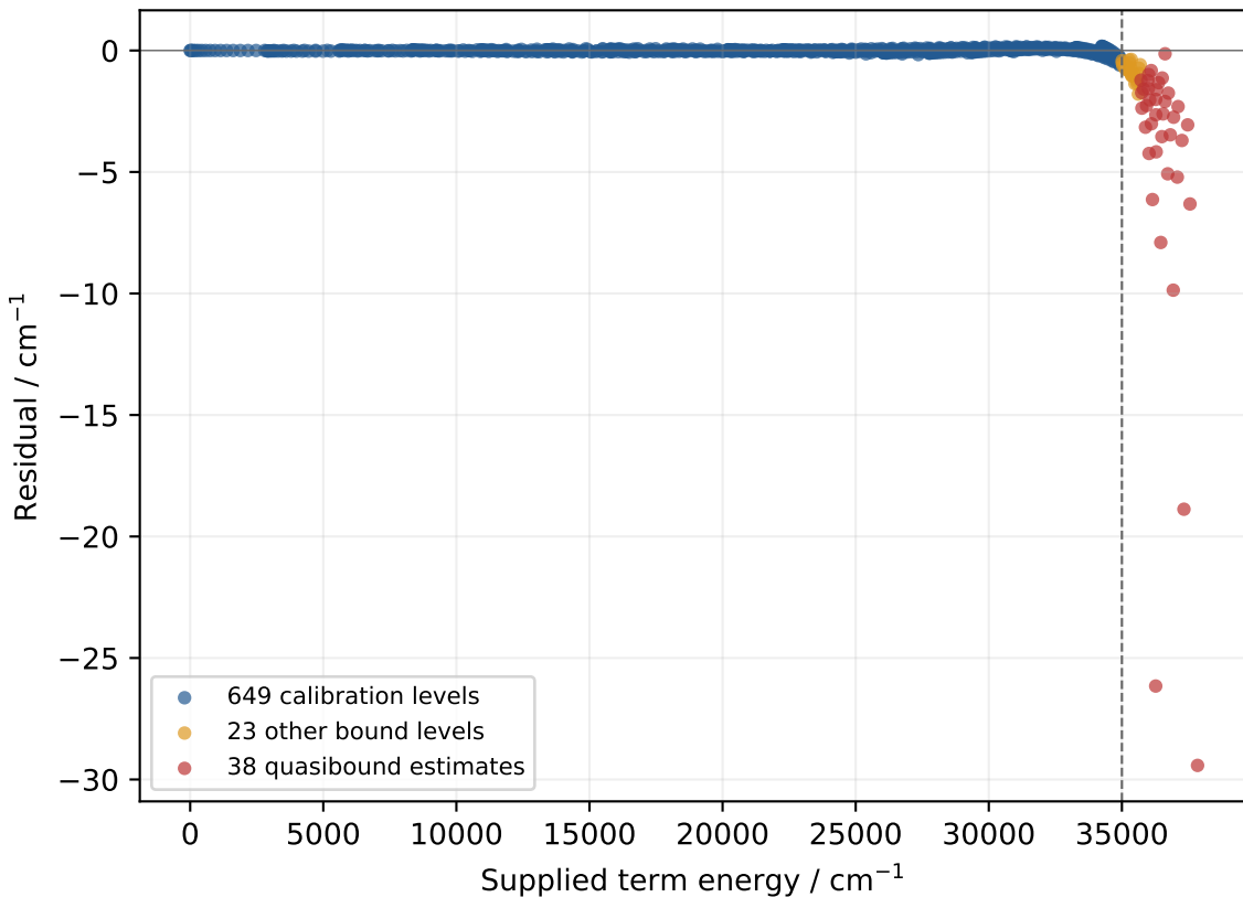
All 710 levels; only blue points were fitted
