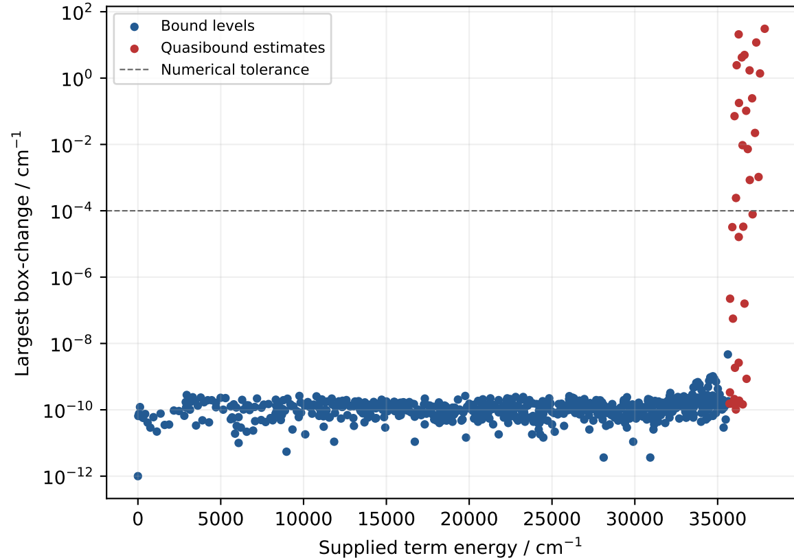
Radial-box convergence
