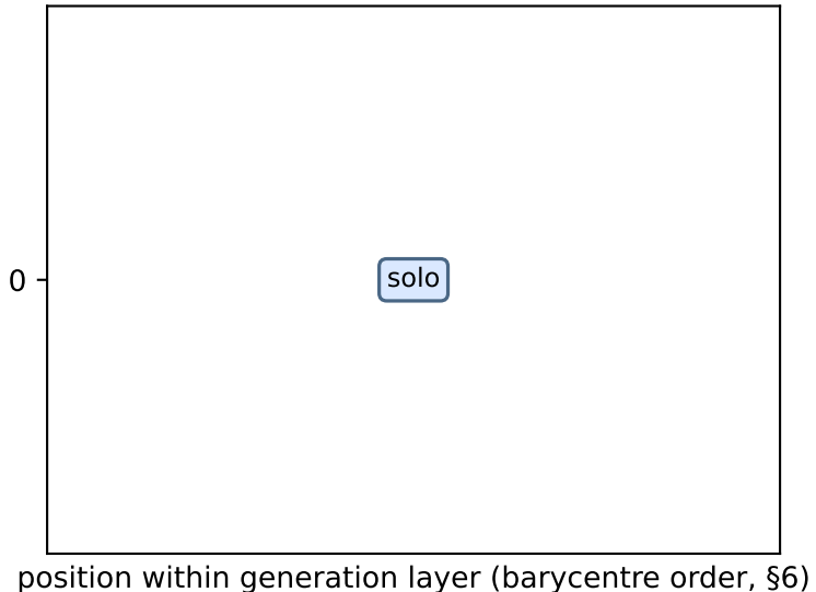
Cluster 2 (1 person)
