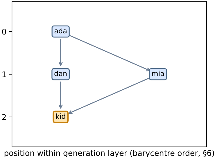
Cluster 1 (4 persons)
