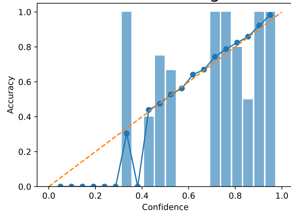
Retained - Forget 1 %
