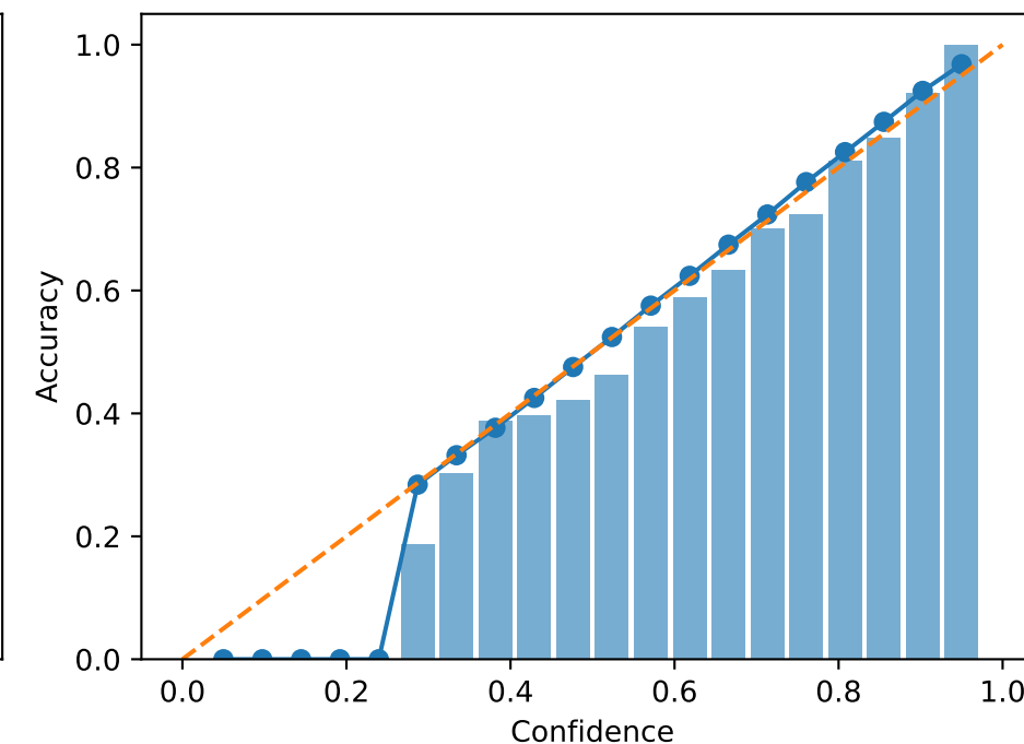
GradDiff - Retain 99%
