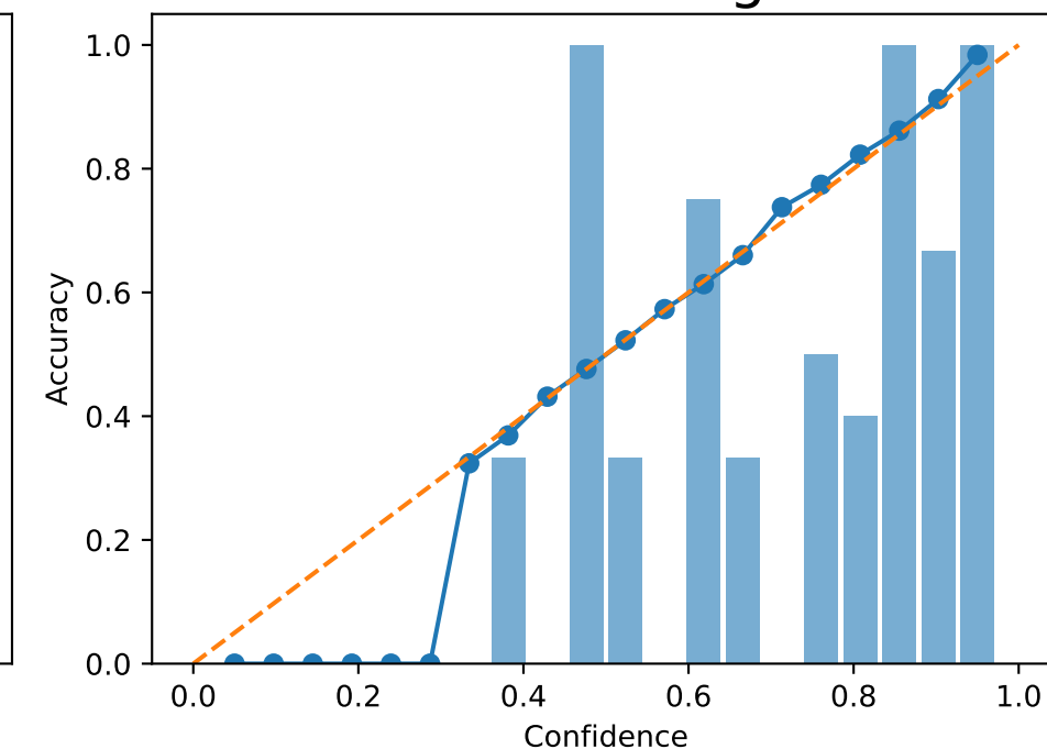
GradDiff - Forget 1 %
