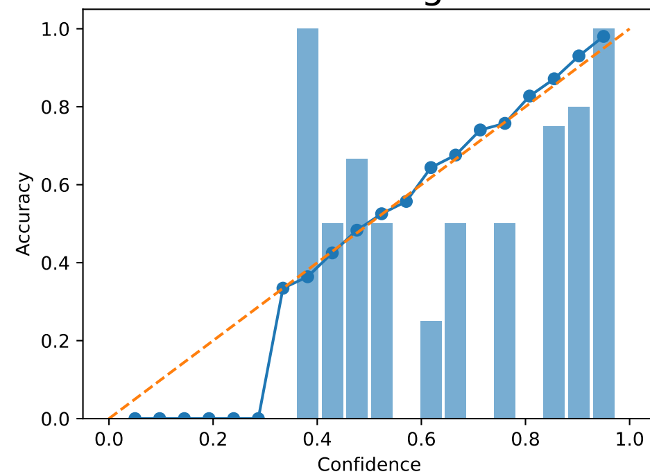
Retained - Forget 1 %
