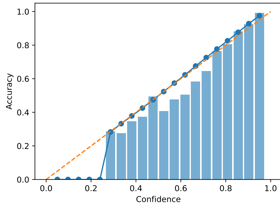
Retained - Retain 99%
