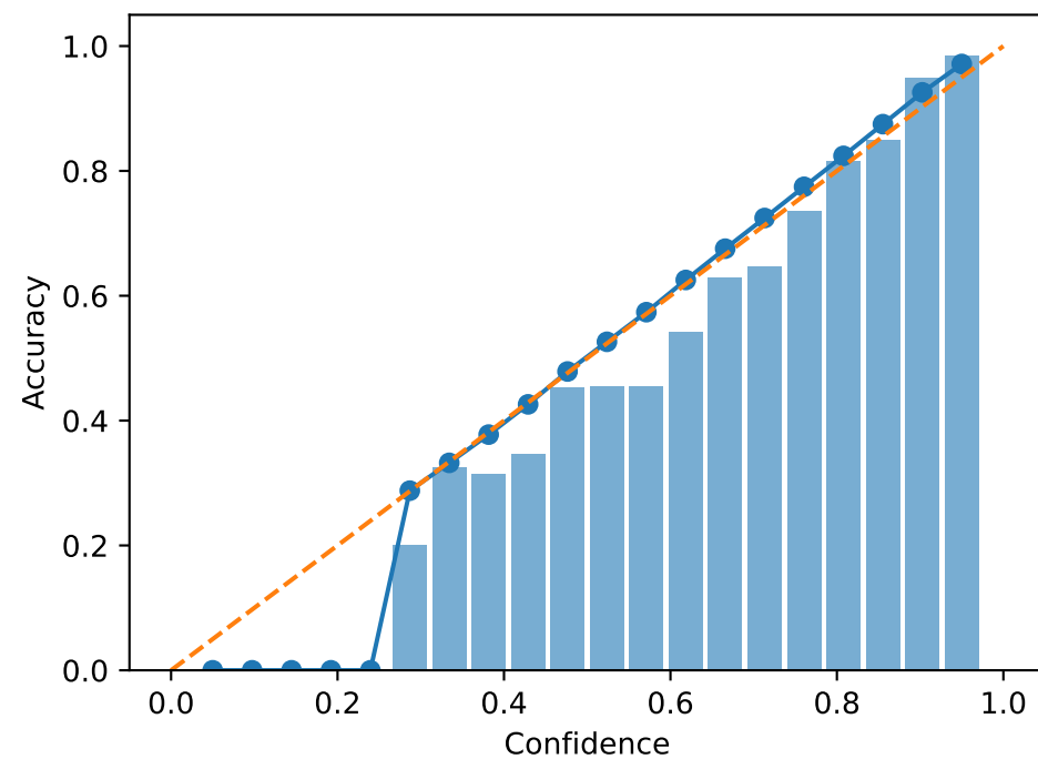
Retained - Retain 99%
