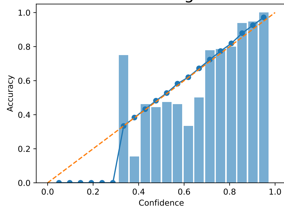
Retained - Forget 5 %
