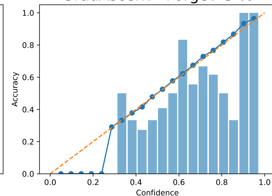
GradDiff - Forget 5 %
