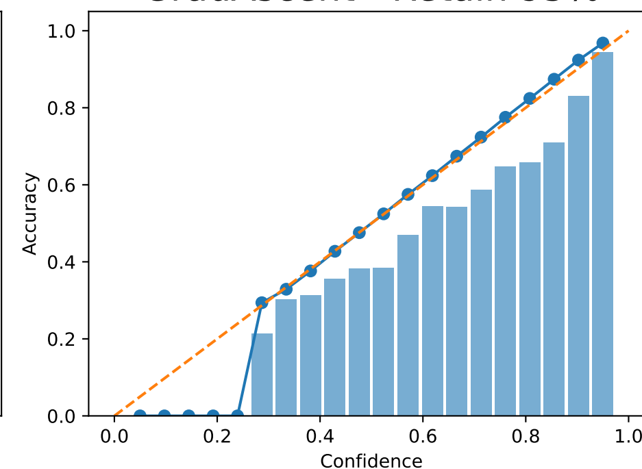
GradDiff - Retain 95%
