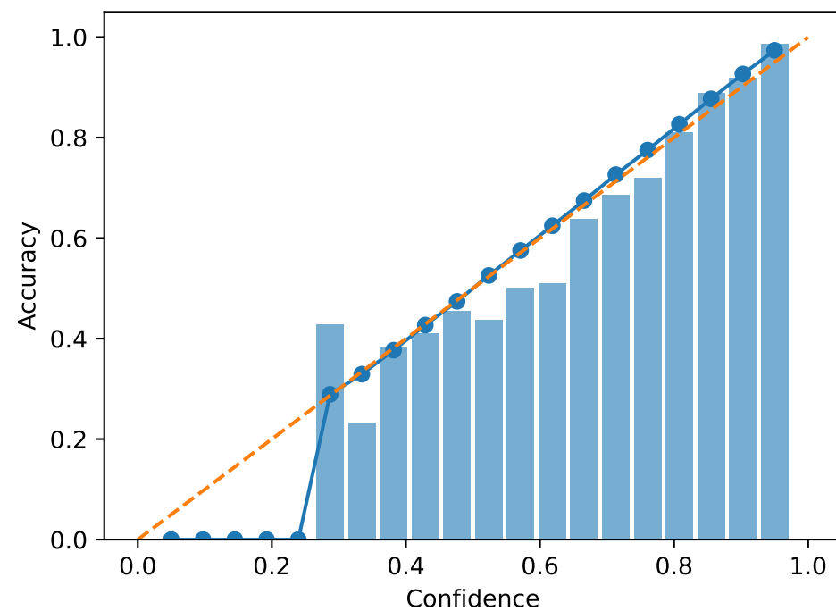
Retained - Retain 95%
