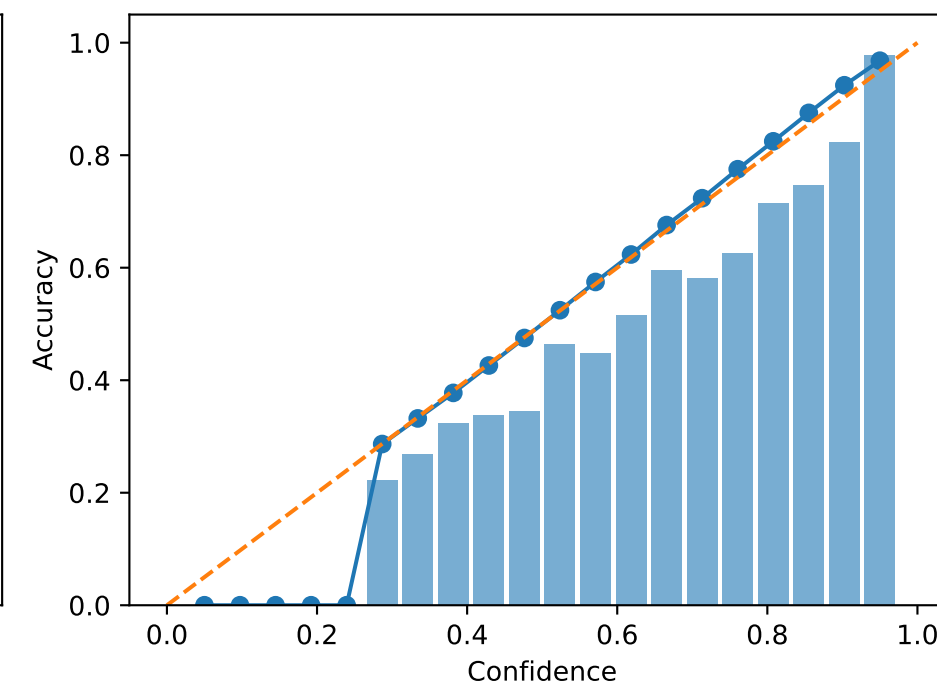
NPO - Retain 95%
