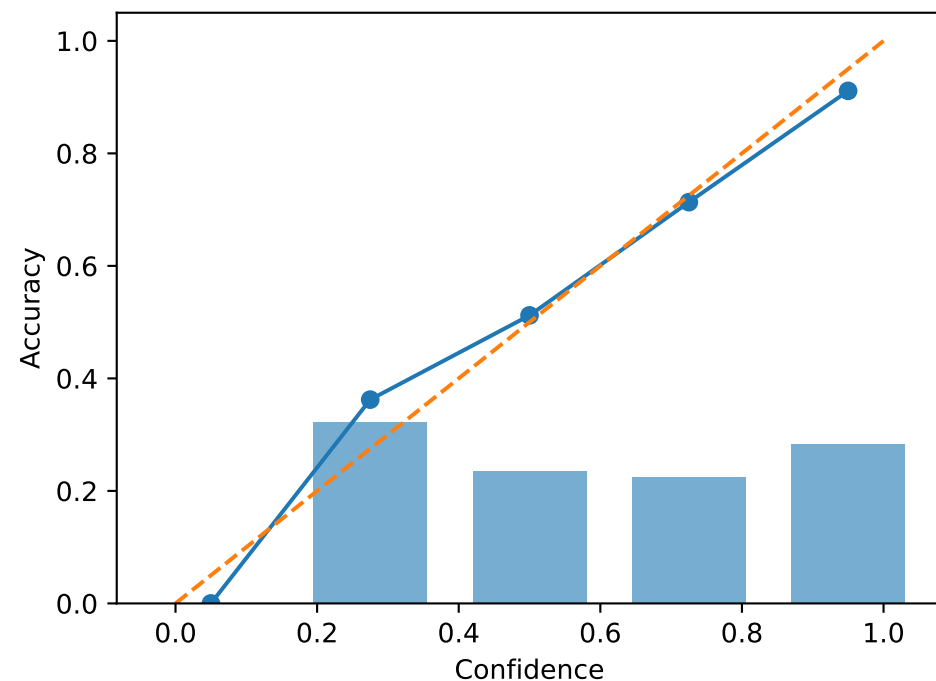
Full Finetuned - Retain 95%
