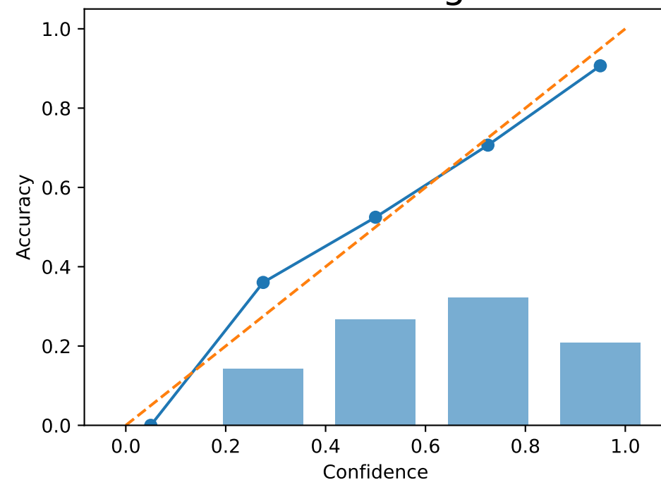
Full Finetuned - Forget 5 %
