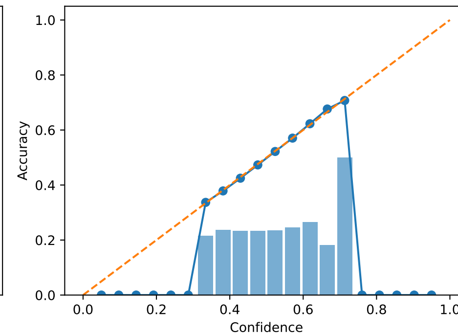
GradDiff - Retain 90%
