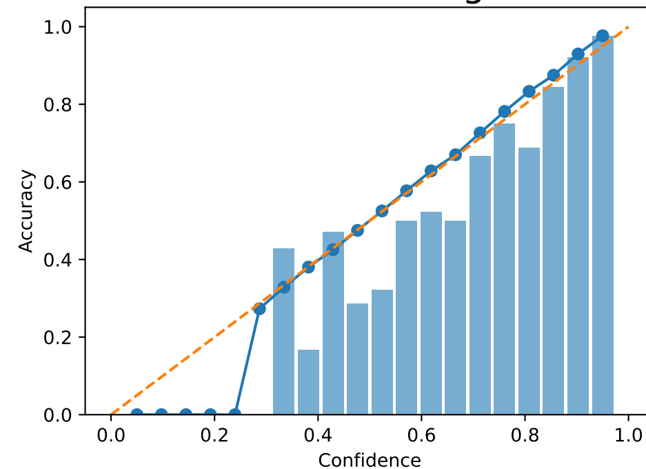
Retained - Forget 10 %
