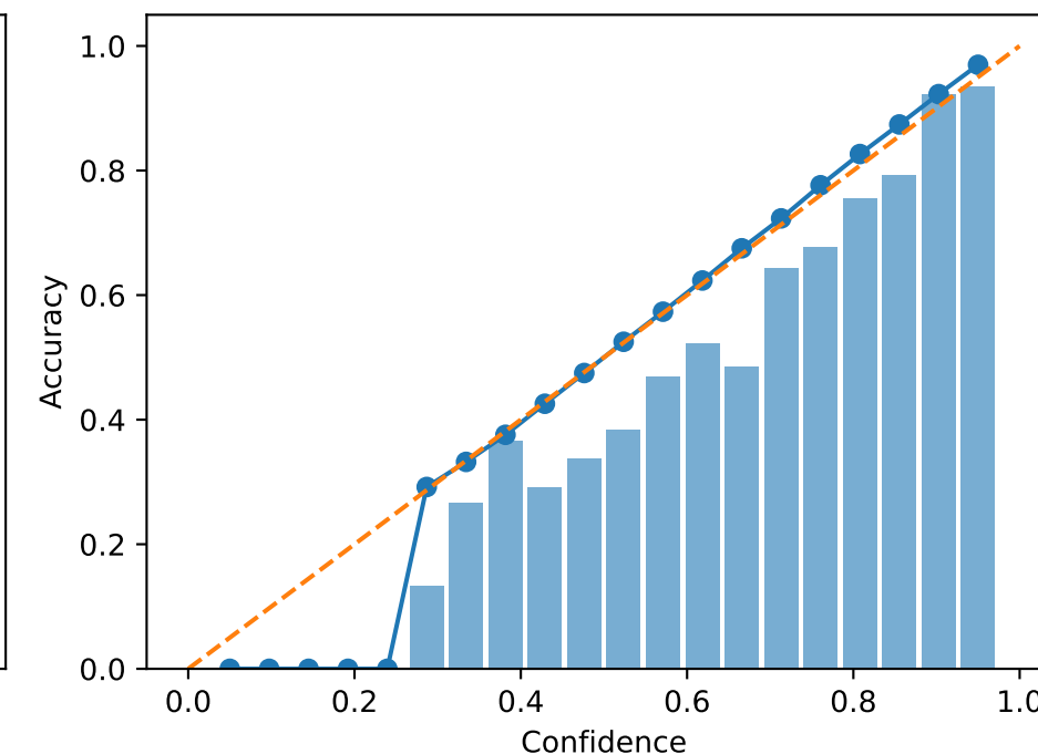
DPO - Retain 90%
