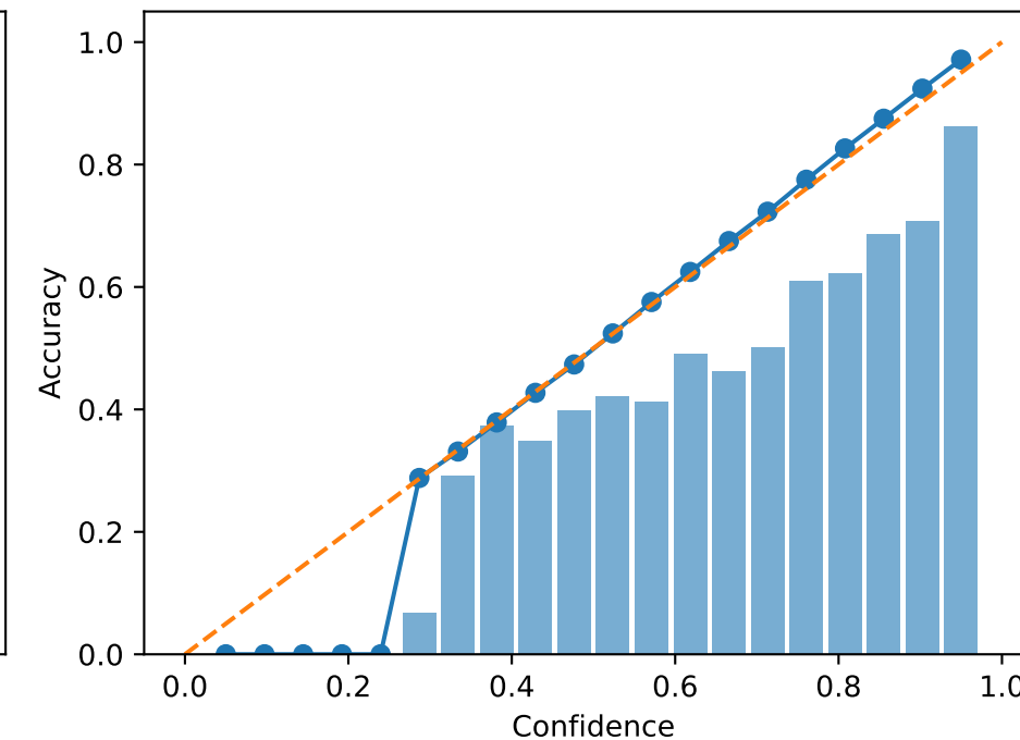
NPO - Retain 90%
