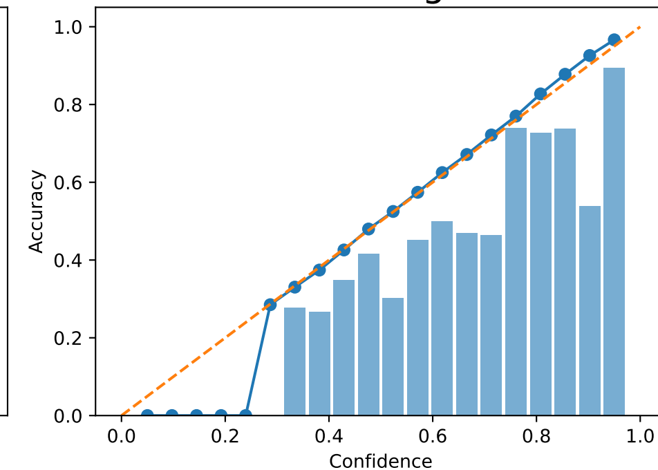
NPO - Forget 10 %
