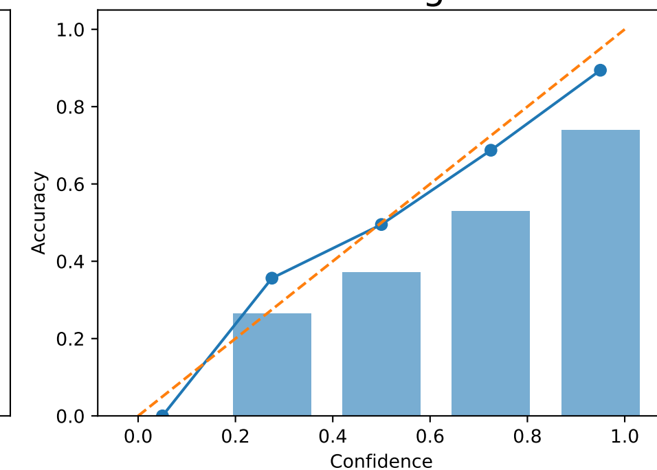
NPO - Forget 10 %
