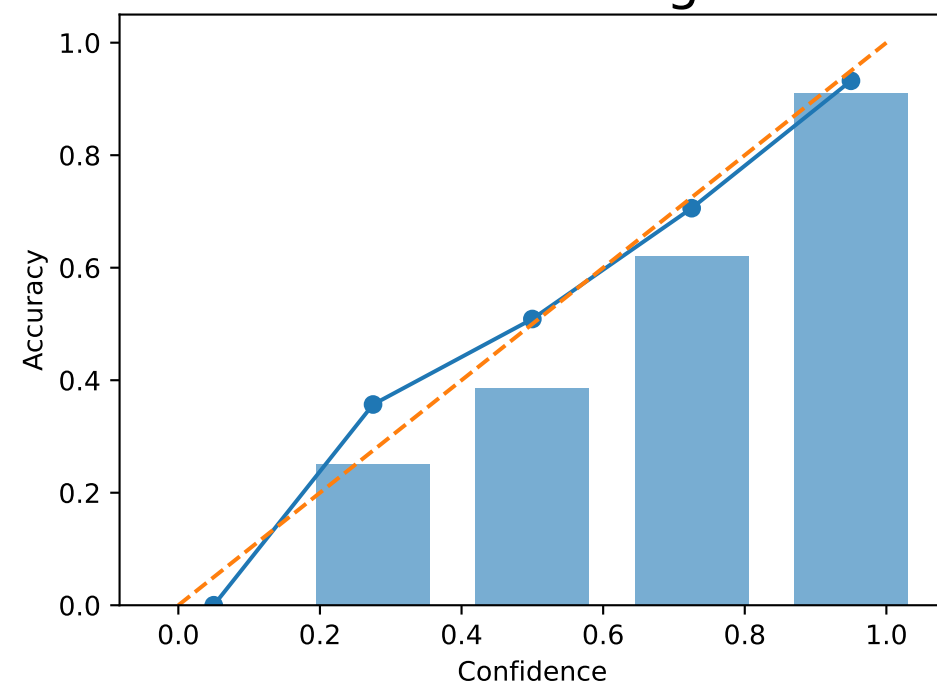
Retained - Forget 10 %
