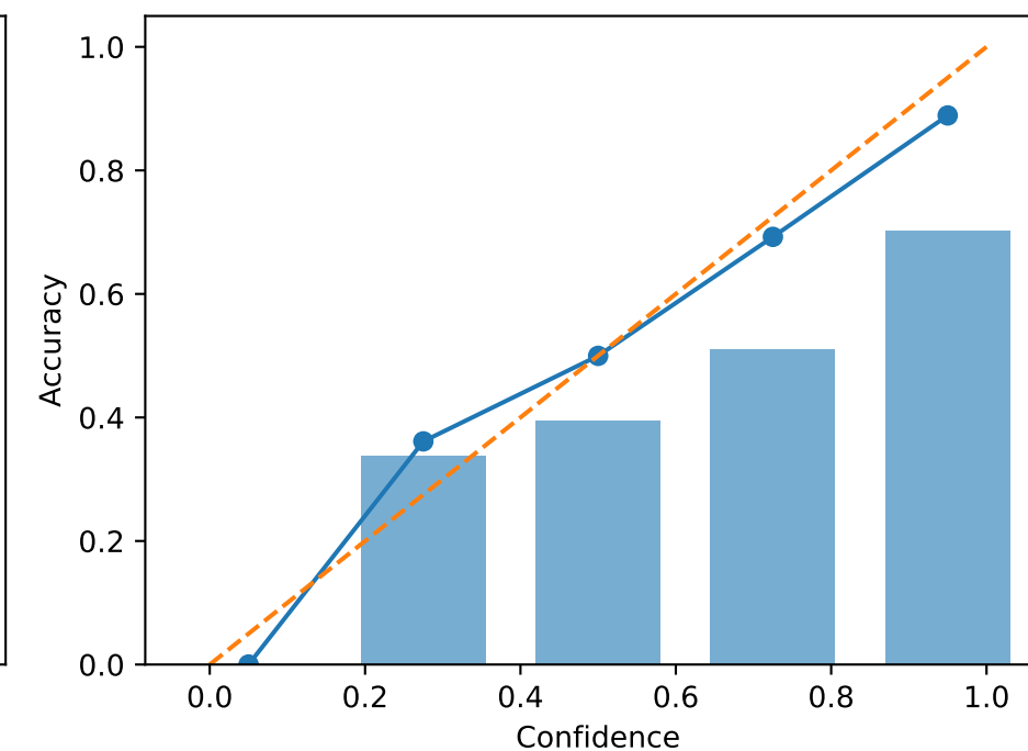
NPO - Retain 90%
