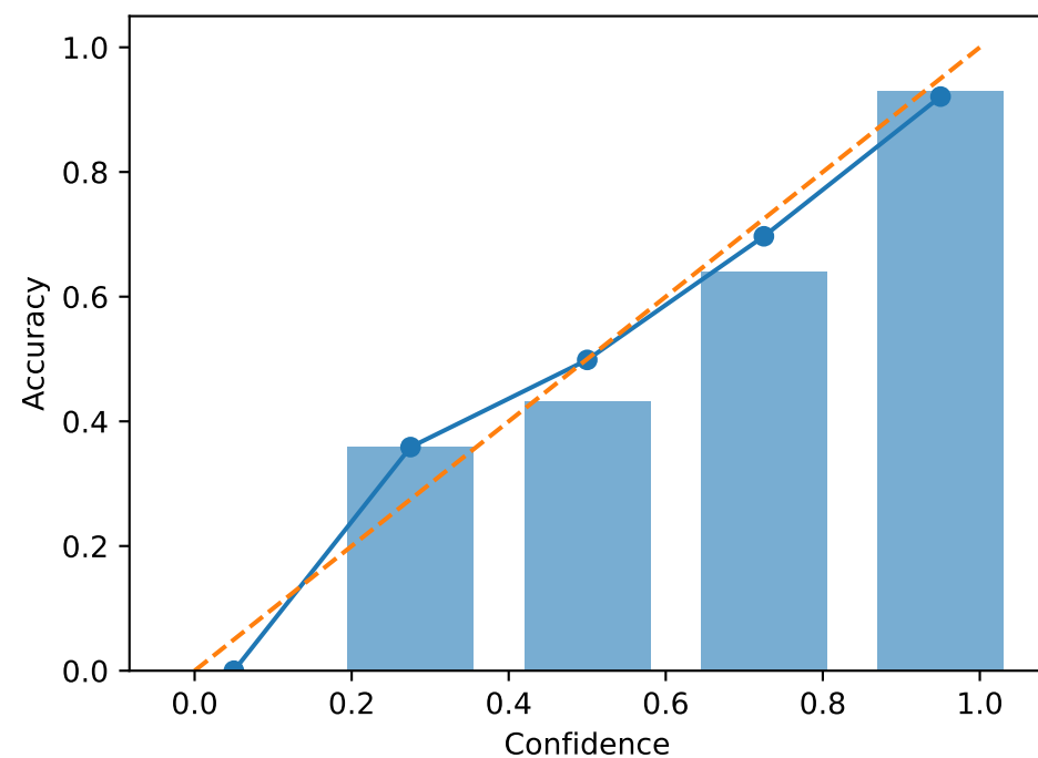
Retained - Retain 90%
