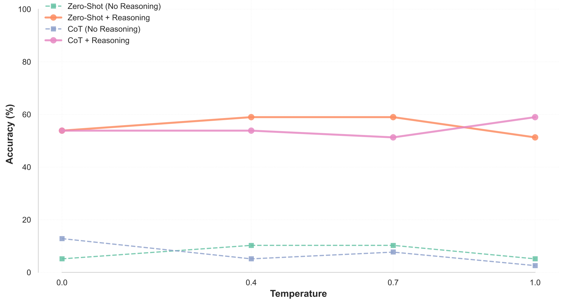
Model Performance Across Temperature Settings
