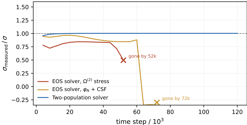
Density ratio 10^3 : what a short run would have reported
