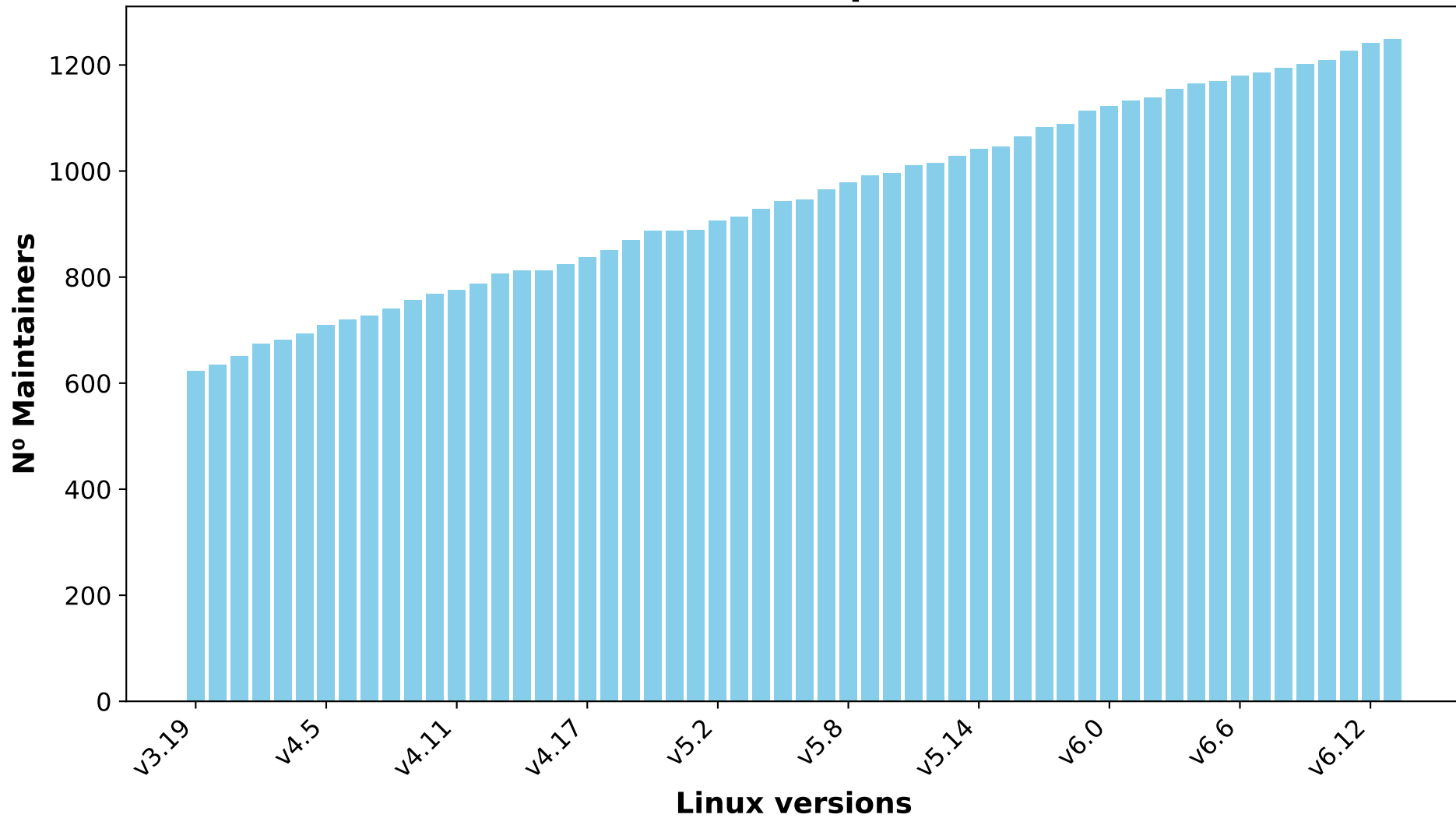
Number of Maintainers per Linux versions
