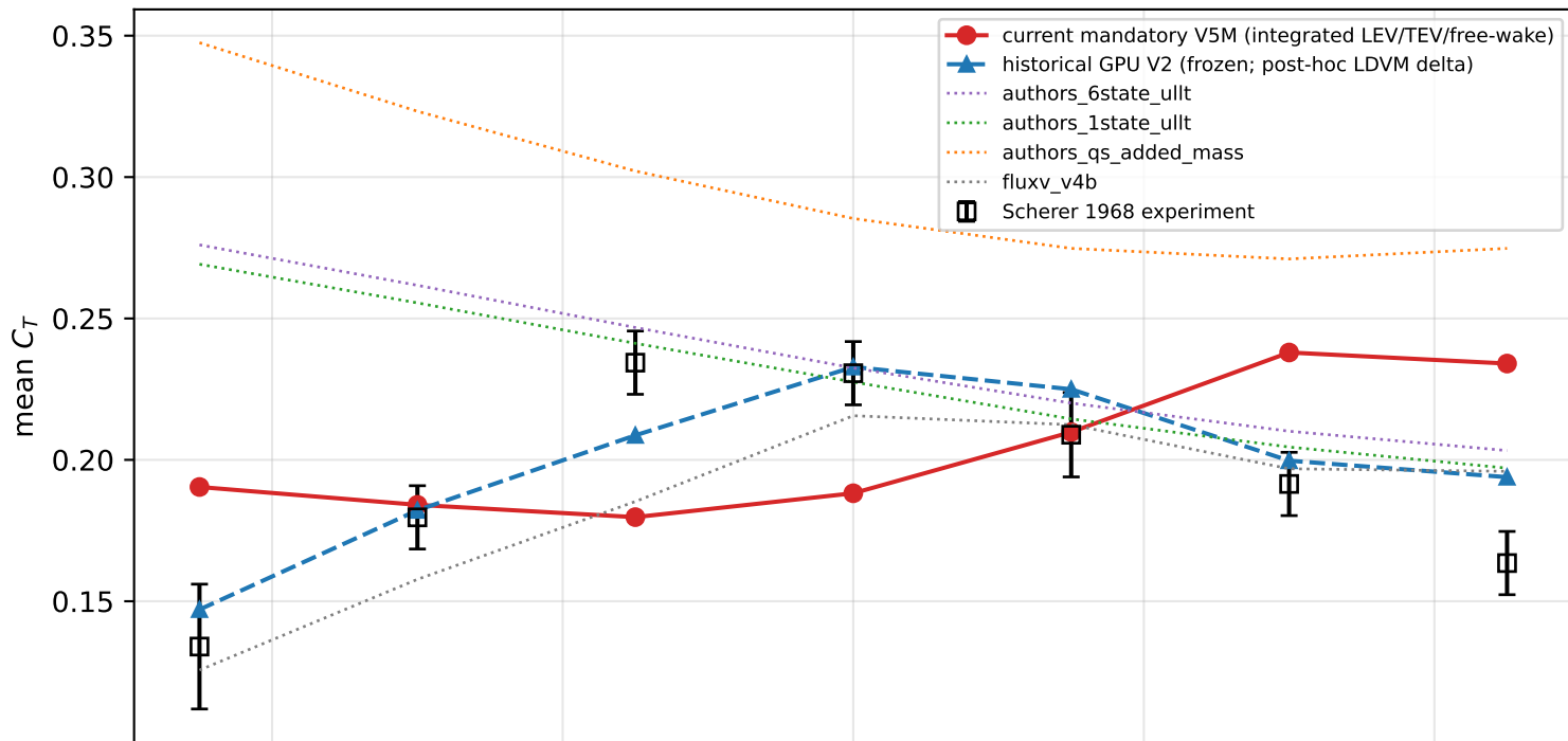
Izraelevitz et al. (2017) Fig.14 — Scherer 1968 thrust coefficient
