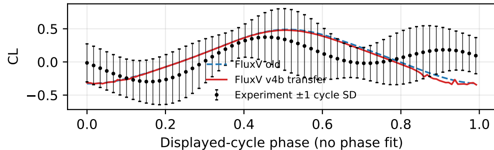
Fig. 10: pitch leading, U=6 m/s, f=1.23 Hz
