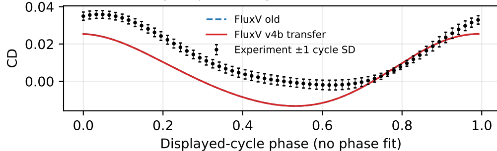
Fig. 11: pitch leading, U=14.8 m/s, f=1.23 Hz
