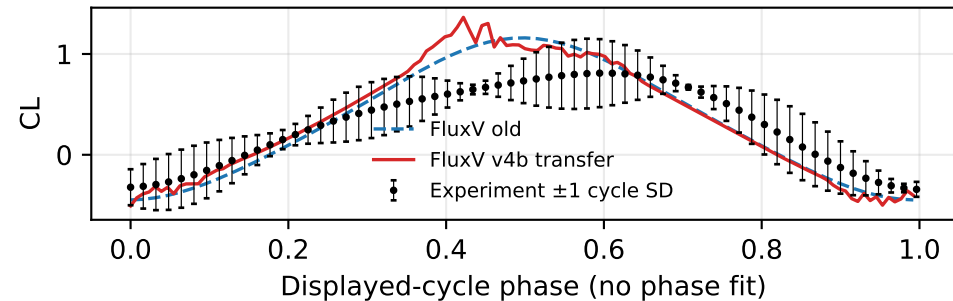
Fig. 13: pitch lagging, U=9.4 m/s, f=1.23 Hz
