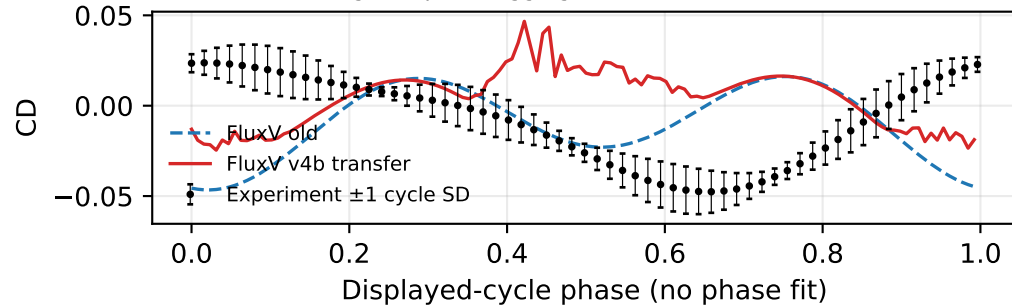
Fig. 13: pitch lagging, U=9.4 m/s, f=1.23 Hz
